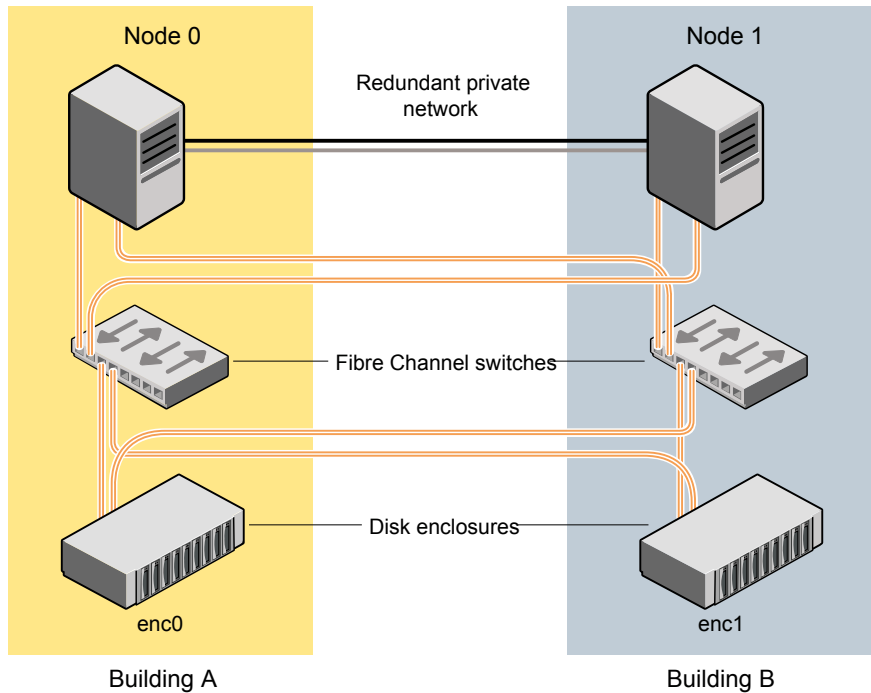
Figure 43-5 Typical arrangement of a 2-node campus cluster
