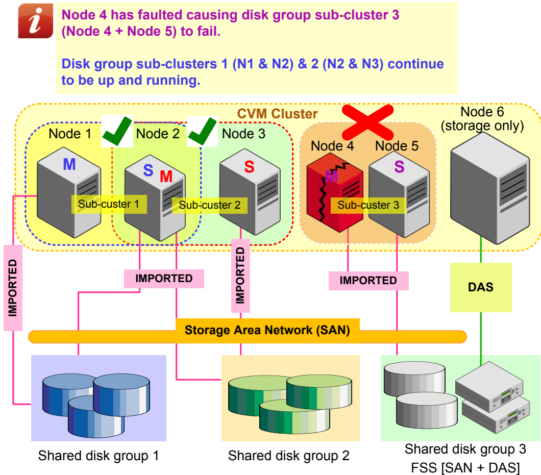
Figure 6-14 Failure management within disk group sub-clusters
