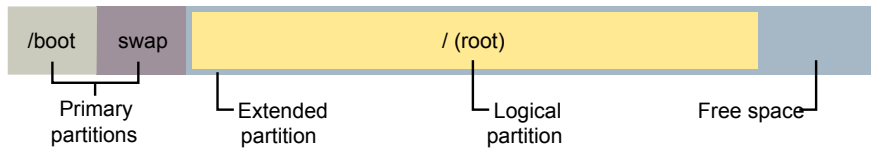
Figure 44-8 Boot and swap configured on two primary partitions, and no free space in the extended partition
