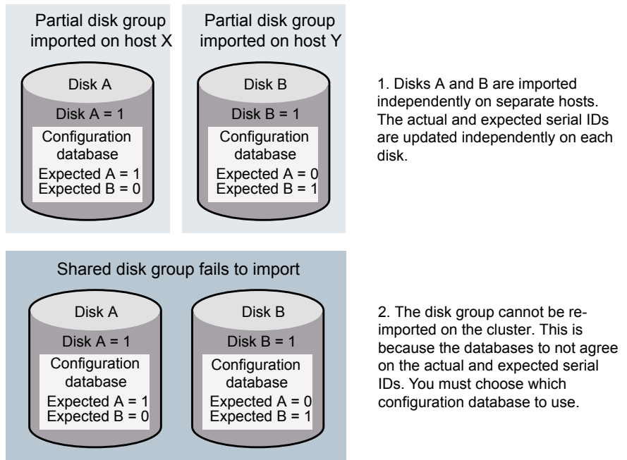
Figure 43-7 Example of a true serial split brain condition that cannot be resolved automatically
