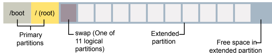
Figure 44-12 Boot and swap configured on two primary partitions, and no more available logical partitions
