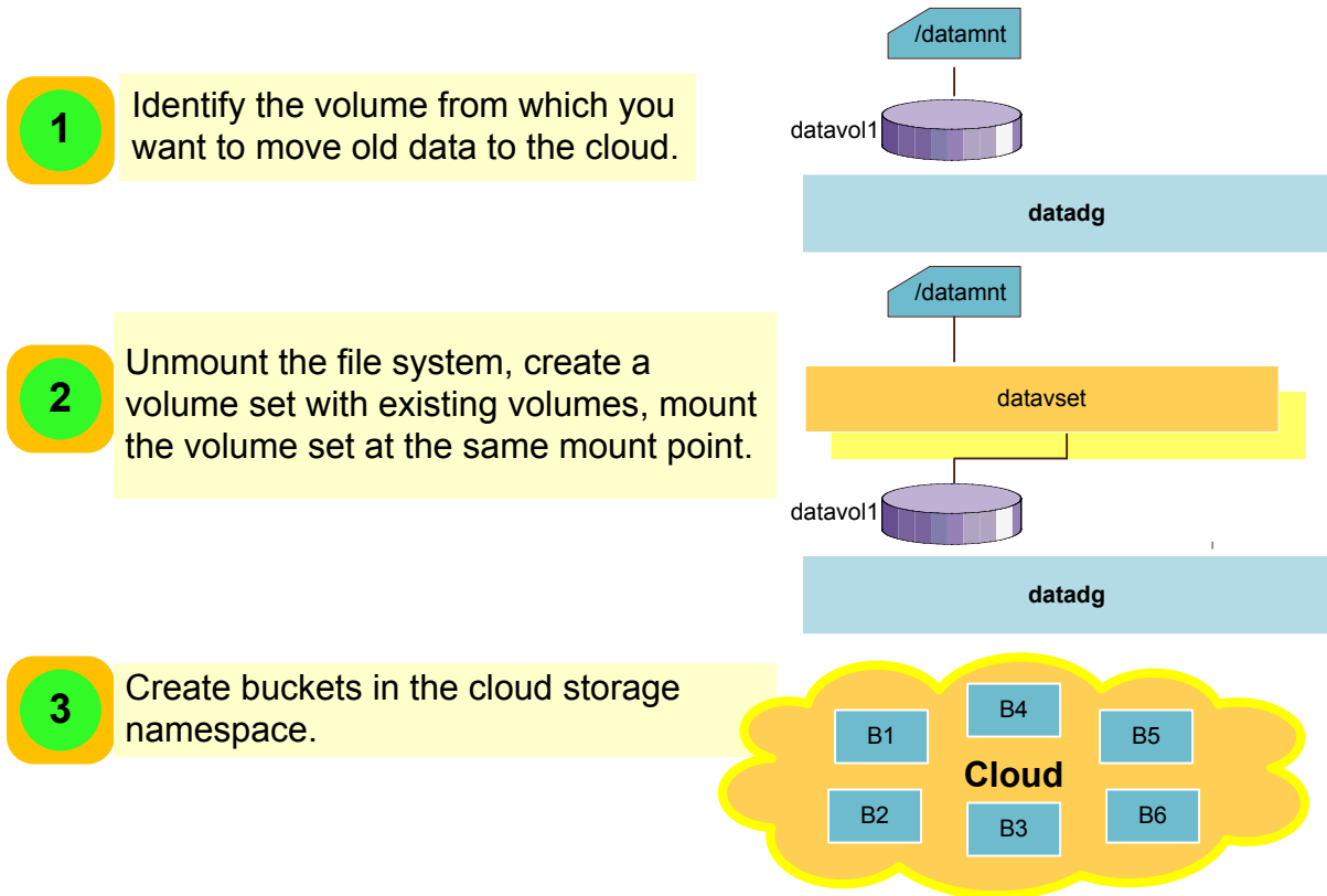
Figure 42-1 S3 Connector - How it works
