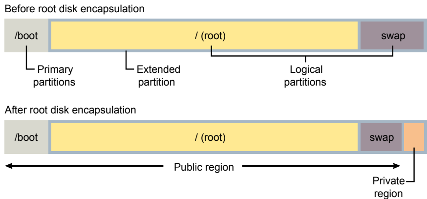
Figure 44-4 Boot configured on a primary partition, and root and swap configured in the extended partition
