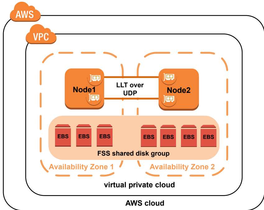
Figure 6-12 FSS in AWS environments
