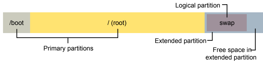
Figure 44-6 Workaround by reconfiguring swap as a logical partition
