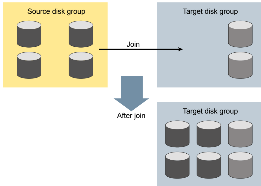
Figure 43-3 Disk group join operation
