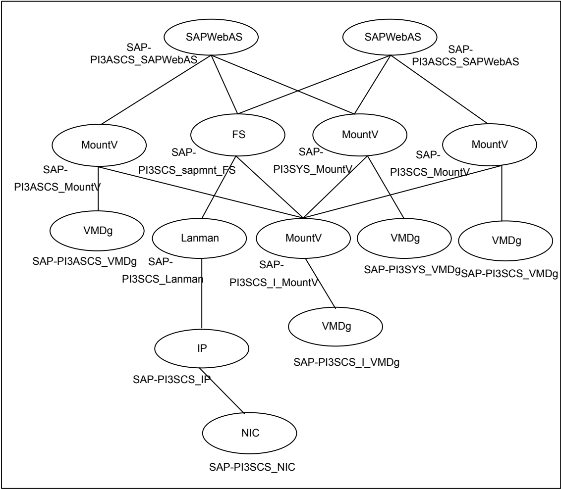
Figure A-6 Sample resource dependency diagram for SAP Central Services Instances service group for Add-In installation Usage Type on a Windows 2008/2012 Server
