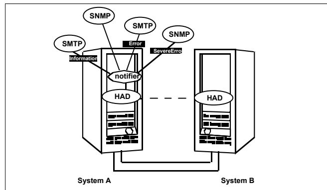
Figure 12-1 VCS event notification: Severity levels
