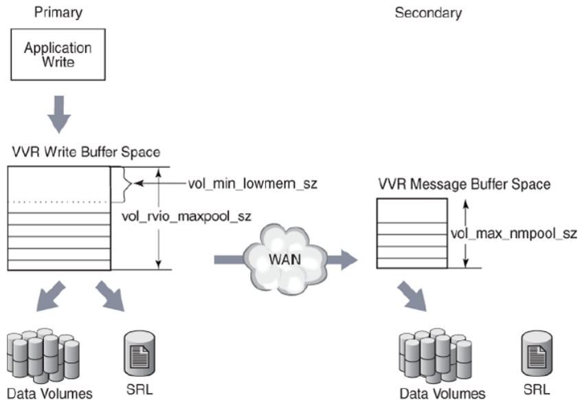
Figure 14-1 How VVR uses buffers between the Primary and Secondary
