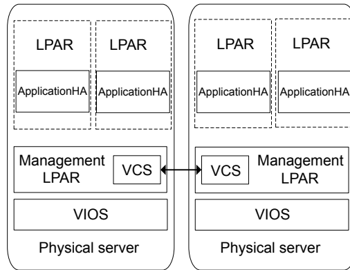
Figure 2-23 VCS in a cluster across LPARs
