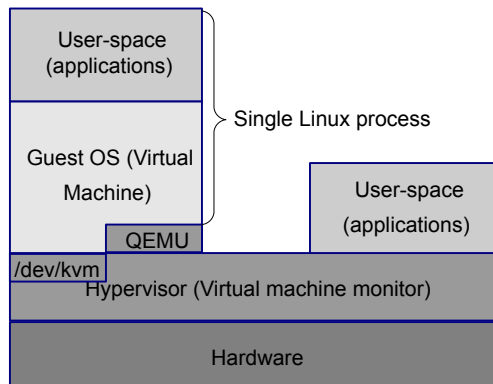
Figure 1-1 KVM process
