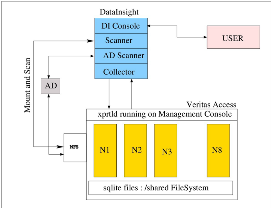
Figure 1-5 High-level design
