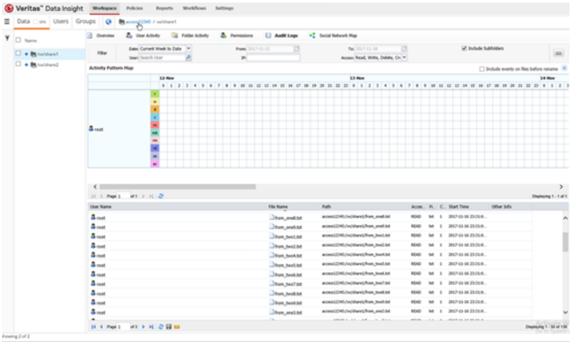
Figure 1-7 Audit information
