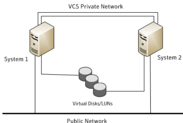
Figure 8-1 Active-Passive configuration
