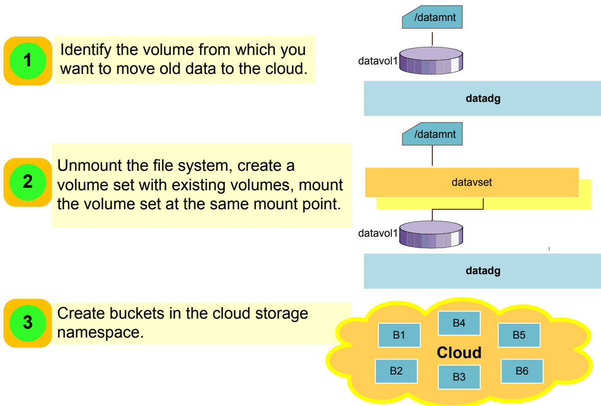
Figure 42-1 How InfoScale migrates data using cloud connectors
