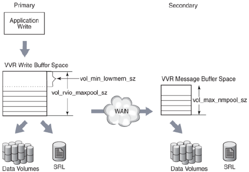
Figure 14-1 How VVR uses buffers between the Primary and Secondary
