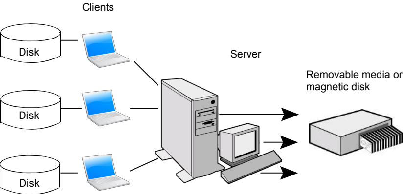
Figure 20-13 Multiplexed backups
