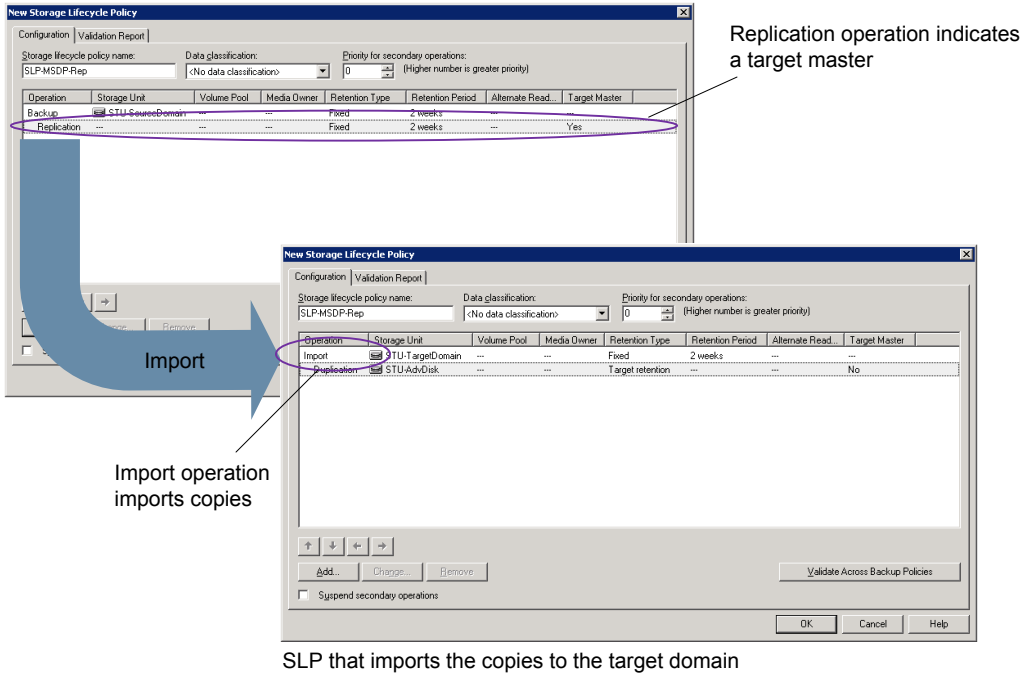
Figure 25-4 Storage lifecycle policy pair required for Auto Image Replication
