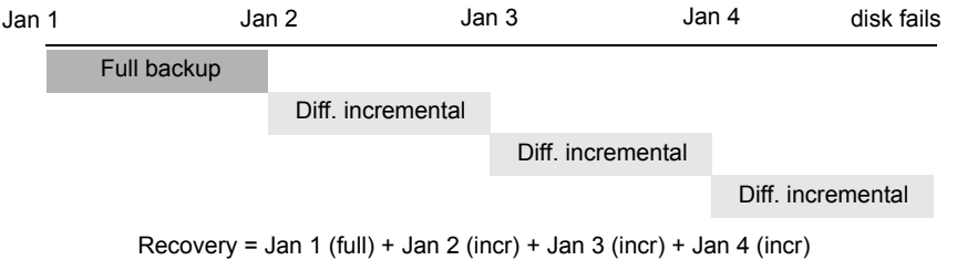
Figure 20-11 Full and differential incremental example
