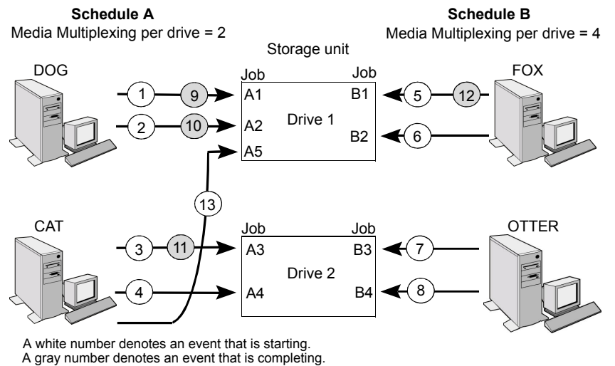
Figure 20-14 Multiplexing process scenario
