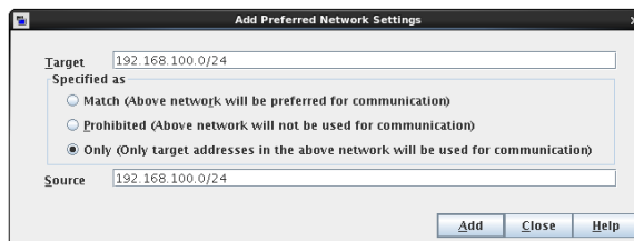
Figure 3-55 Only network selection with the same source binding address
