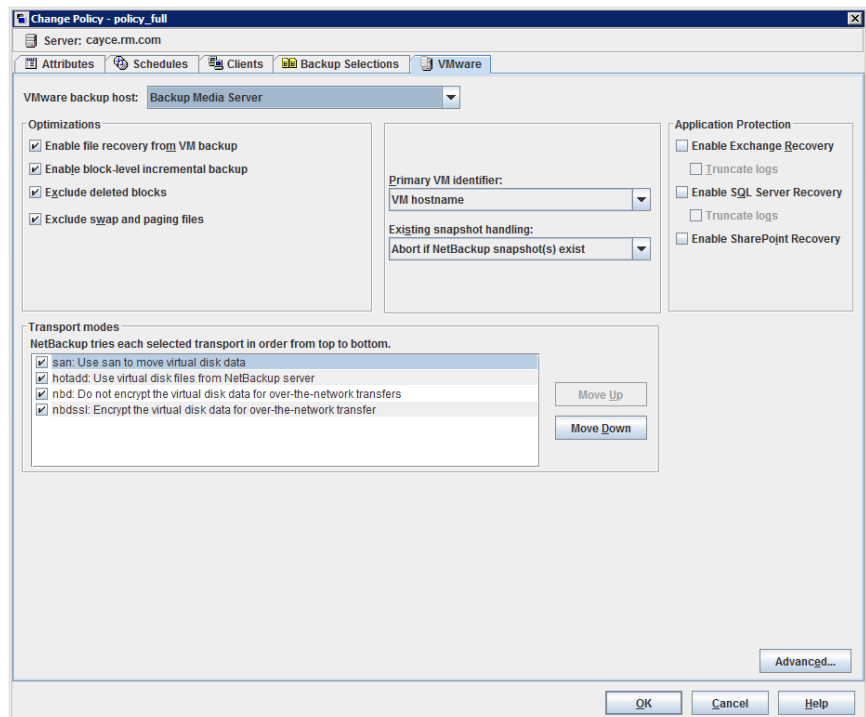
Figure 20-32 VMware tab
