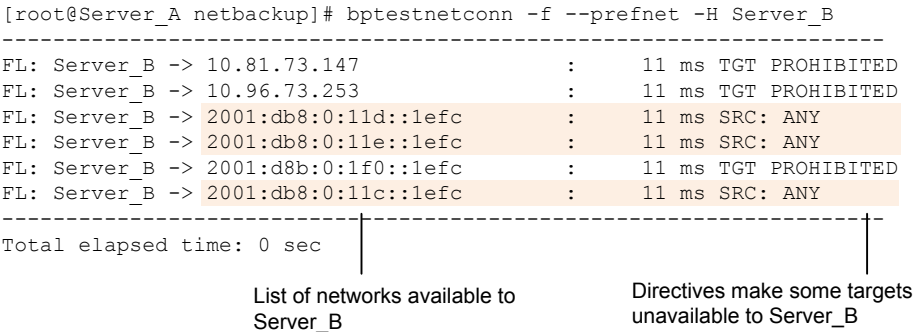
Figure 3-52 bptestnetconn for Server_B with directive
