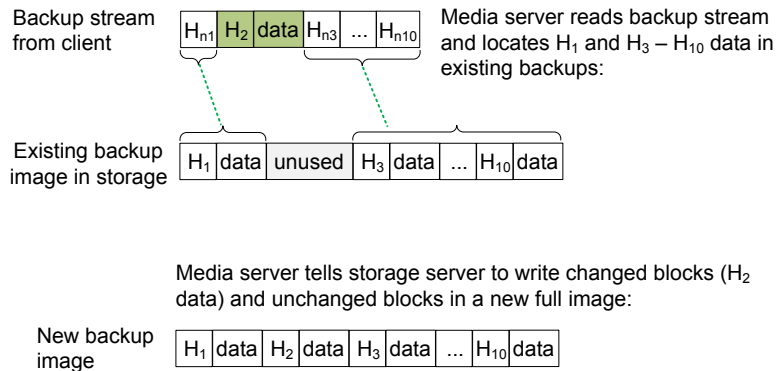
Figure 21-7 NetBackup media server constructs backup image
