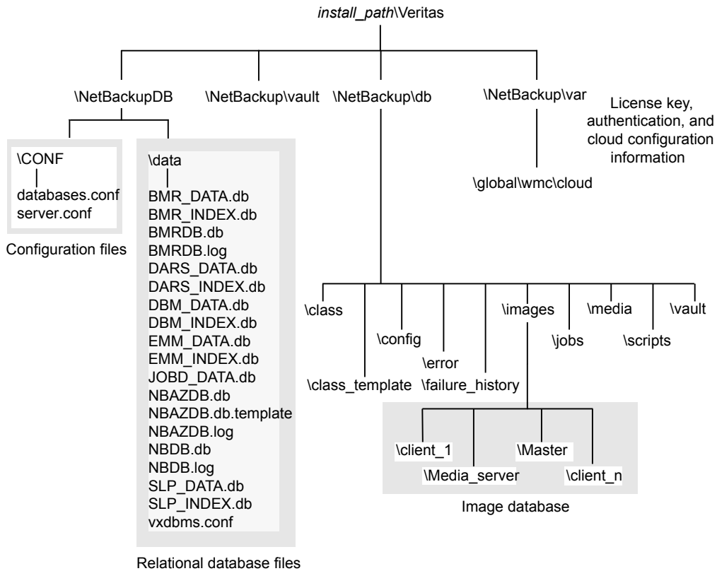
Figure 23-1 Catalog configuration on Windows computers
