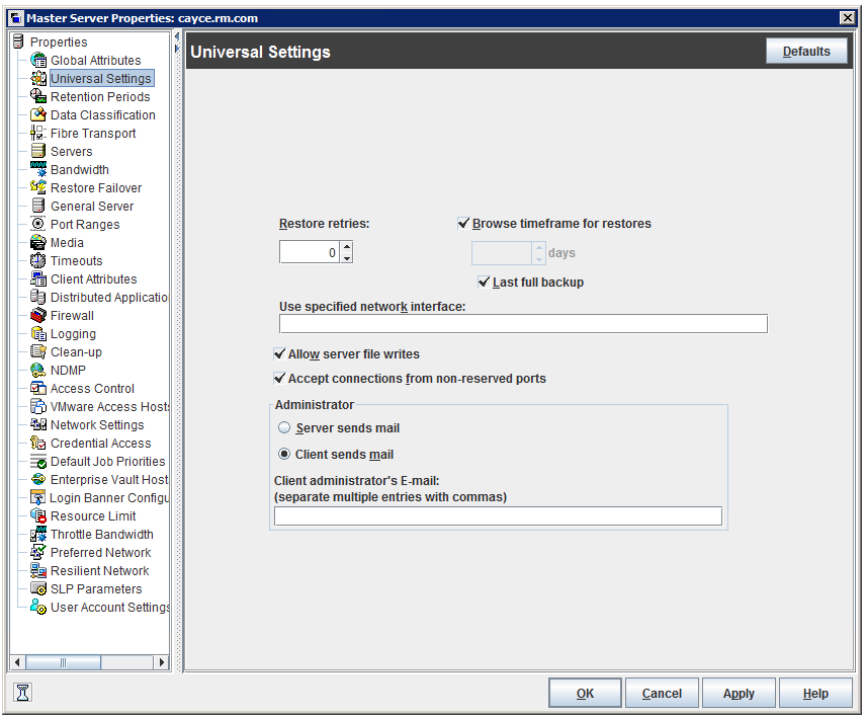
Figure 3-63 Universal Settings dialog box
