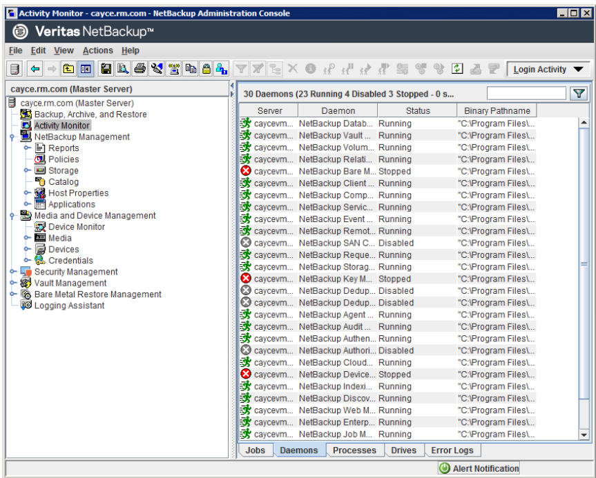
Figure 28-2 The Daemons tab in the Activity Monitor
