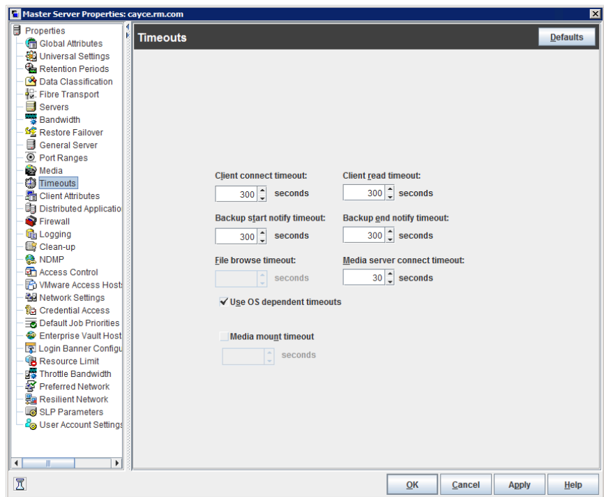
Figure 3-62 Timeouts dialog box
