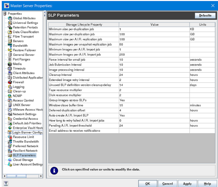
Figure 3-60 SLP Parameters dialog box
