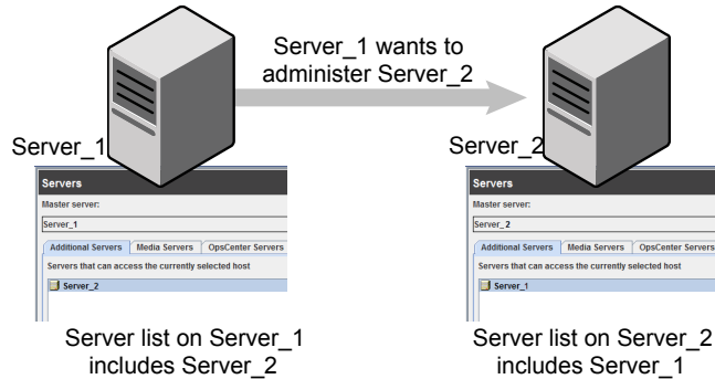
Figure 32-1 Server lists on local server and remote server
