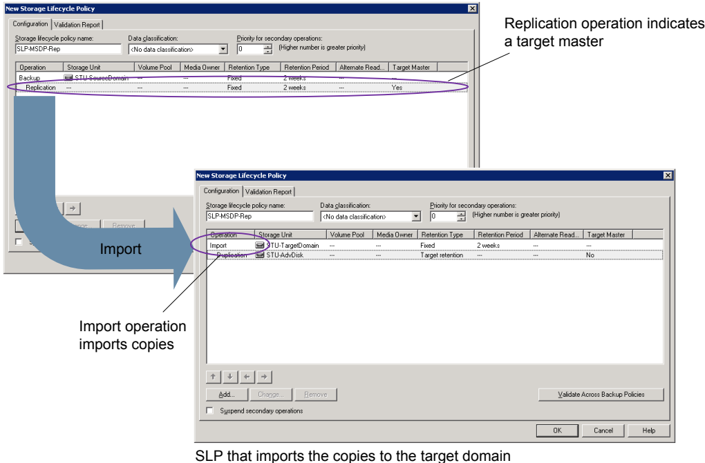
Figure 27-4 Storage lifecycle policy pair required for Auto Image Replication
