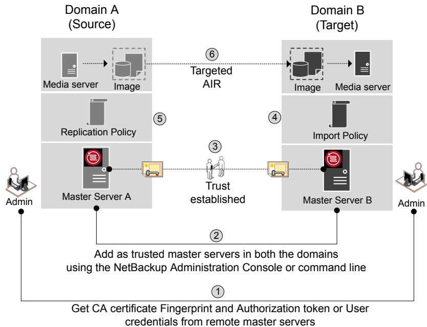
Figure 27-3 Tasks to establish a trust relationship between master servers for targeted A.I.R. using NetBackup CA-signed certificate
