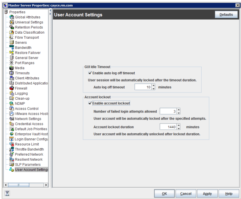
Figure 3-64 User Account Settings dialog box
