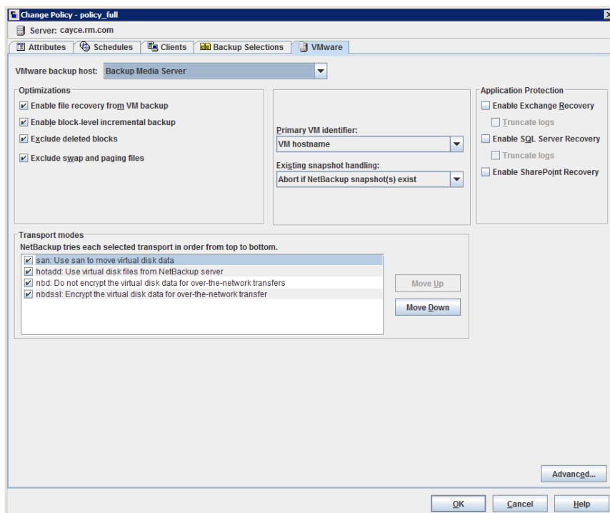
Figure 21-31 VMware tab
