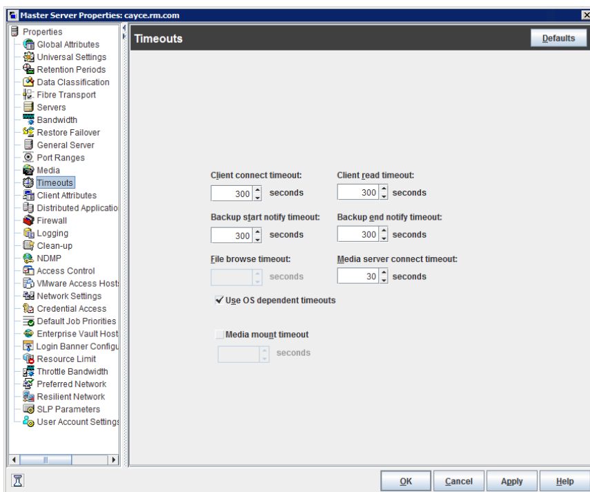
Figure 3-61 Timeouts dialog box
