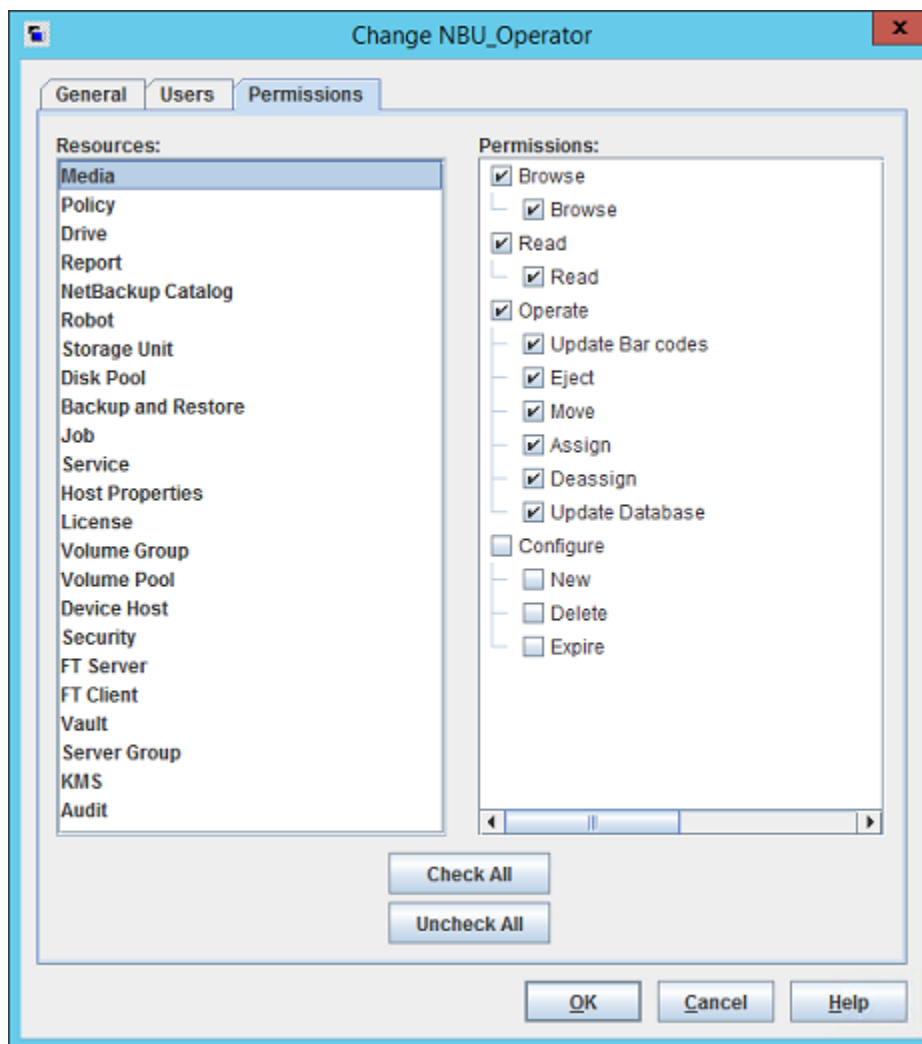
Figure 6-18 Permissions list
