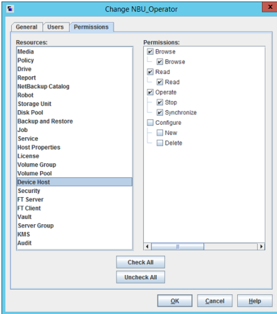
Figure A-17 Authorization objects
