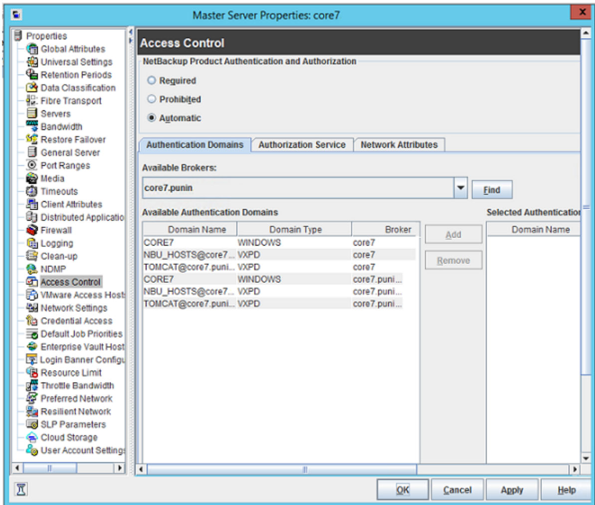
Figure A-11 Cross platform authentication domains
