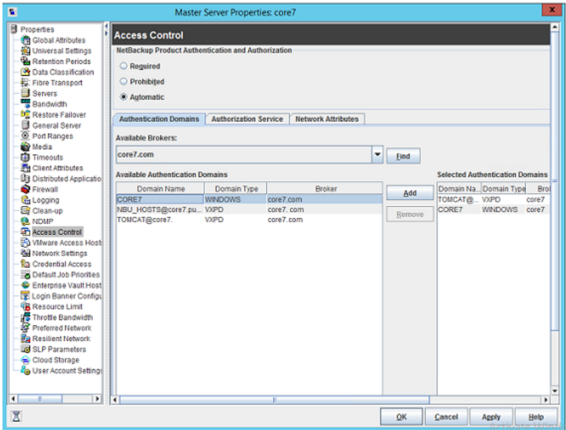
Figure A-1 Access control host properties dialog box
