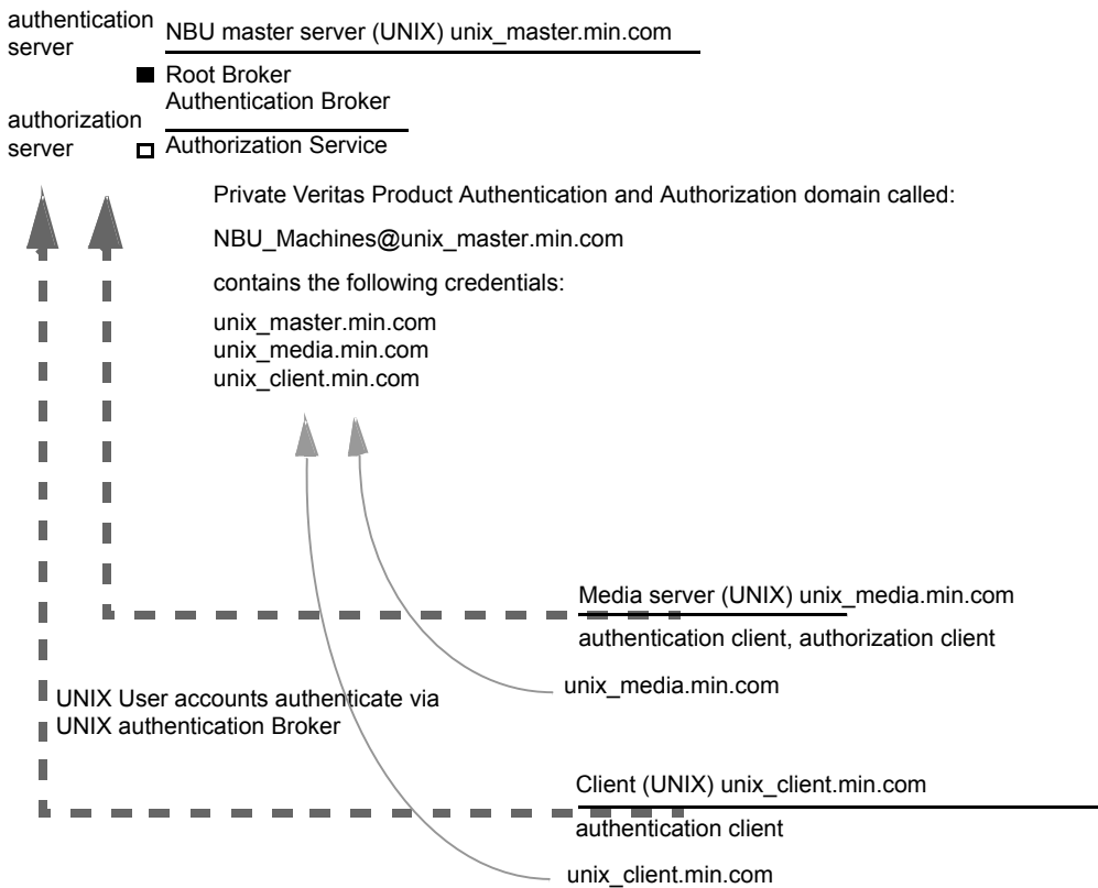
Figure A-9 Example configuration containing UNIX systems only
