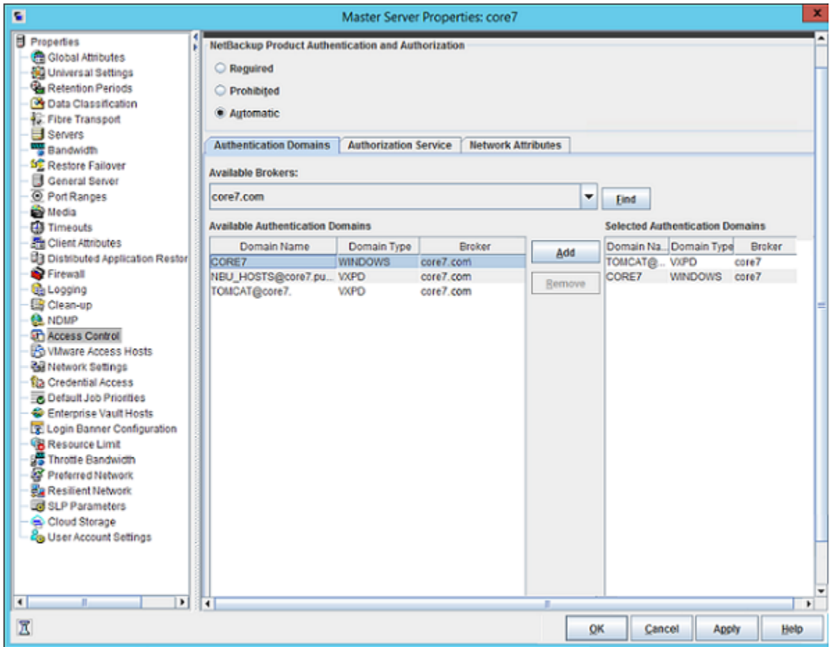
Figure A-5 Authentication Domain tab for client
