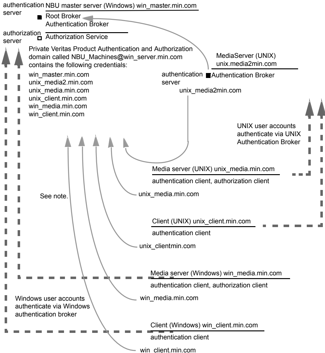
Figure A-12 Example mixed configuration containing a Windows master server
