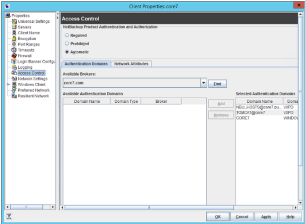
Figure A-4 Access control host properties for the client
