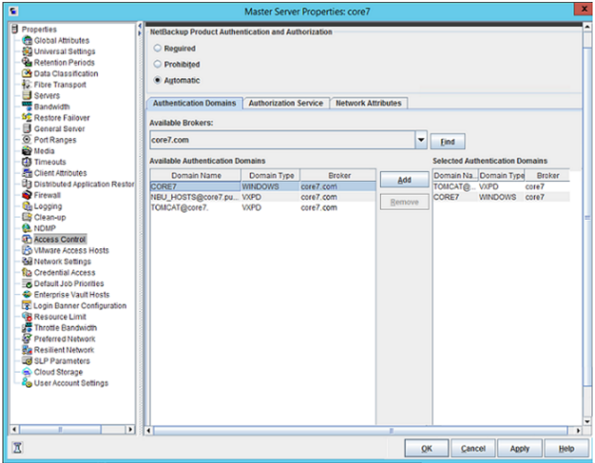
Figure A-2 Authentication Domain tab
