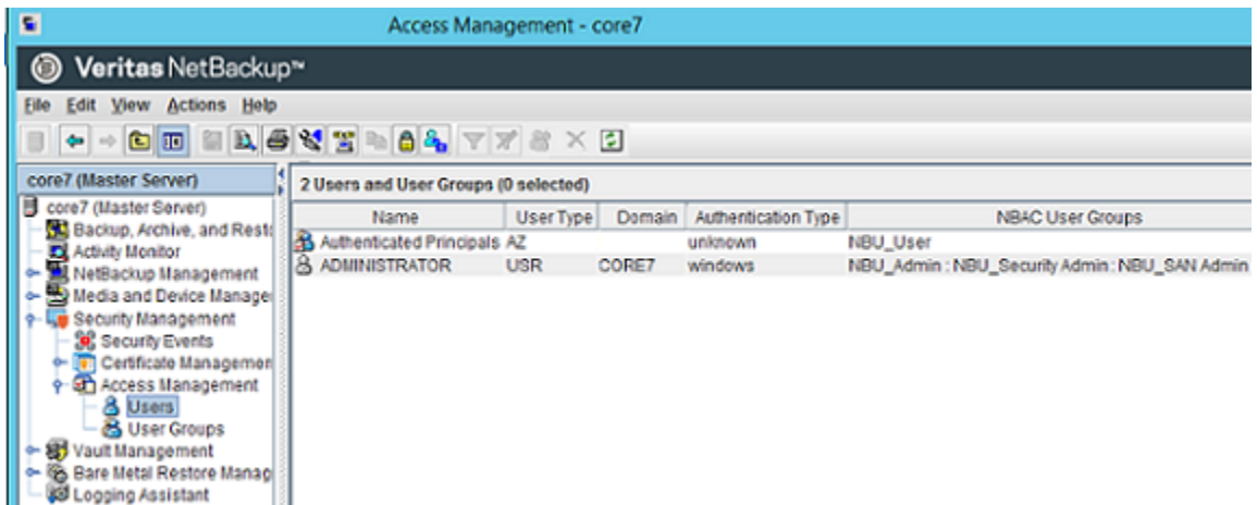
Figure A-13 Individual users
