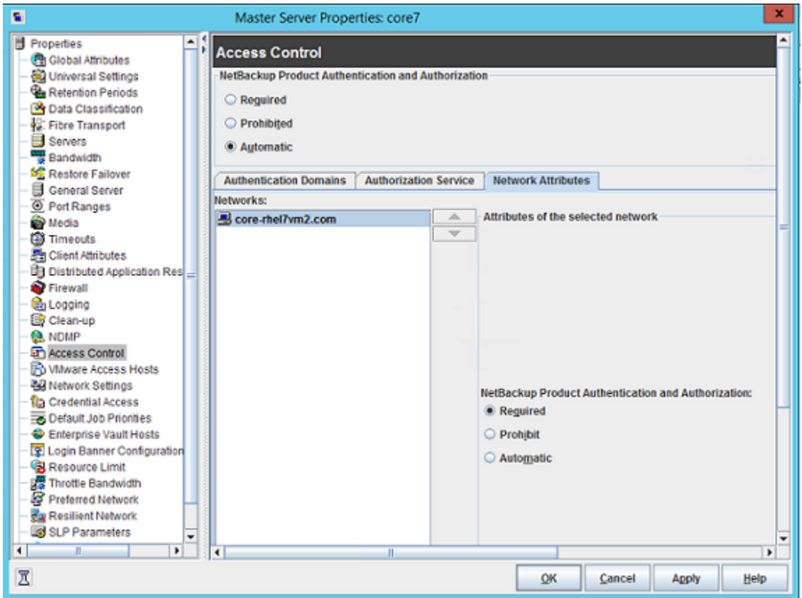
Figure A-6 Network Attributes tab for the client
