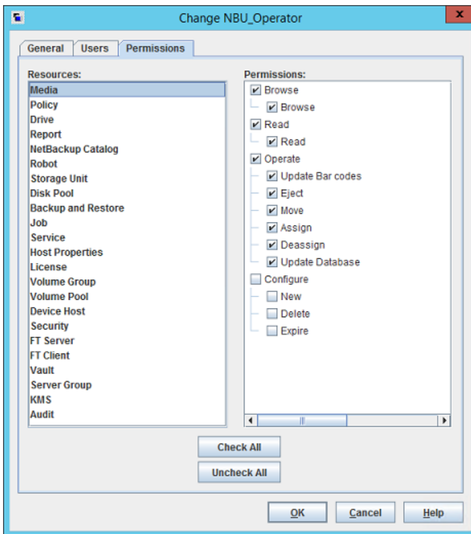
Figure A-18 Permissions list
