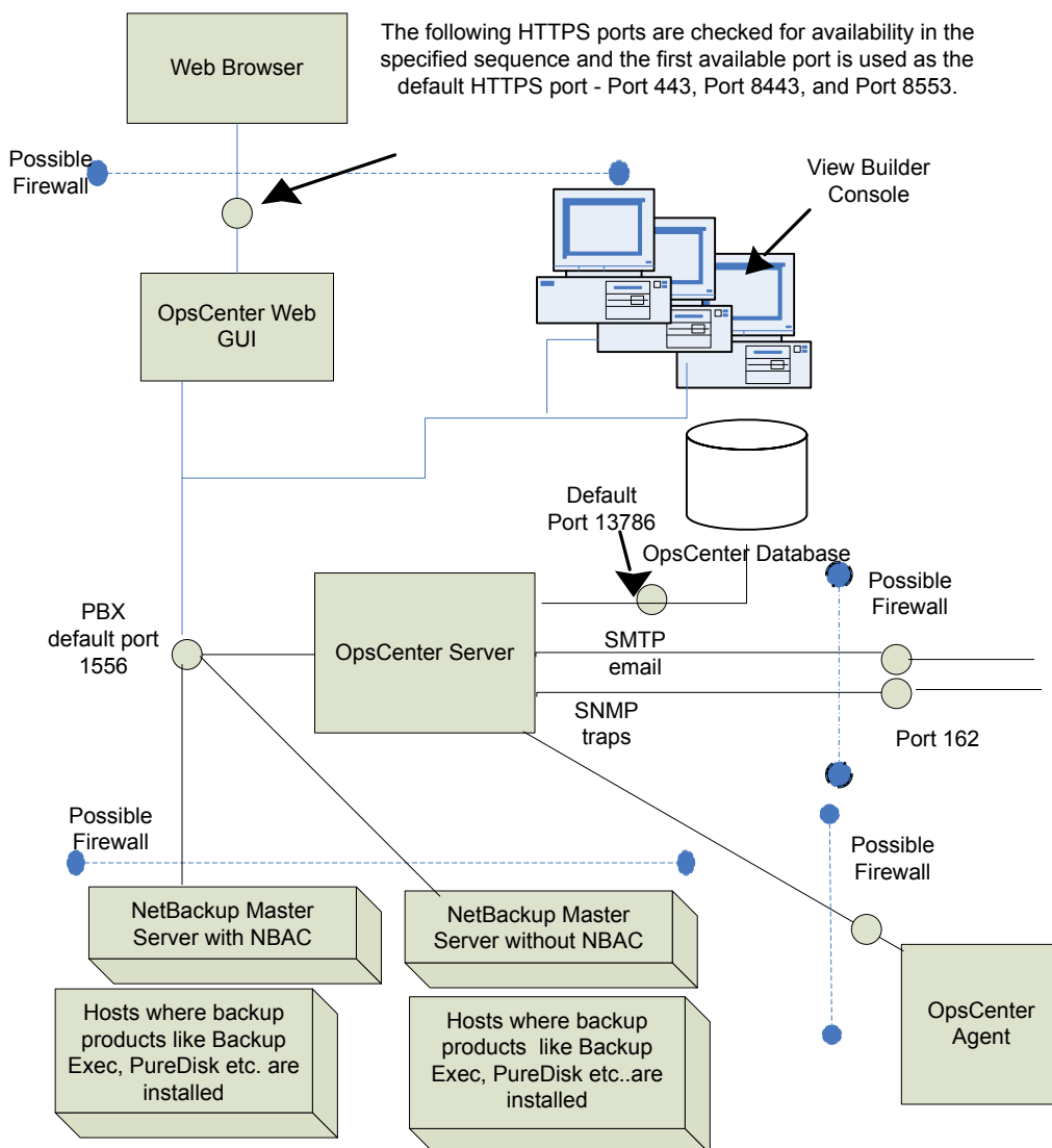
Figure 4-1 Key OpsCenter components and how they communicate
