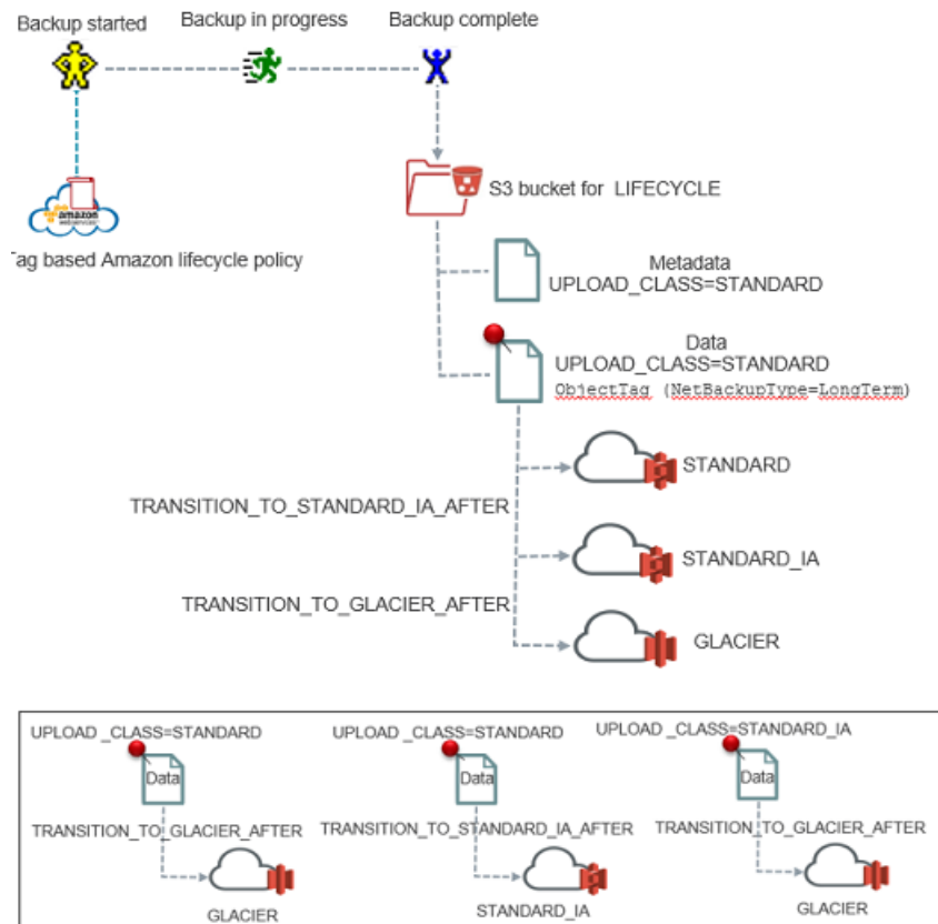
Figure 2-3 Back up process for LIFECYCLE storage class with possible configurations
