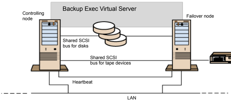
Figure 19-3 Example of a shared bus with tape devices at the end of the bus
