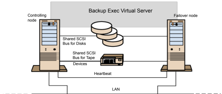
Figure 19-2 Two-node cluster with tape devices on a shared SCSI bus
