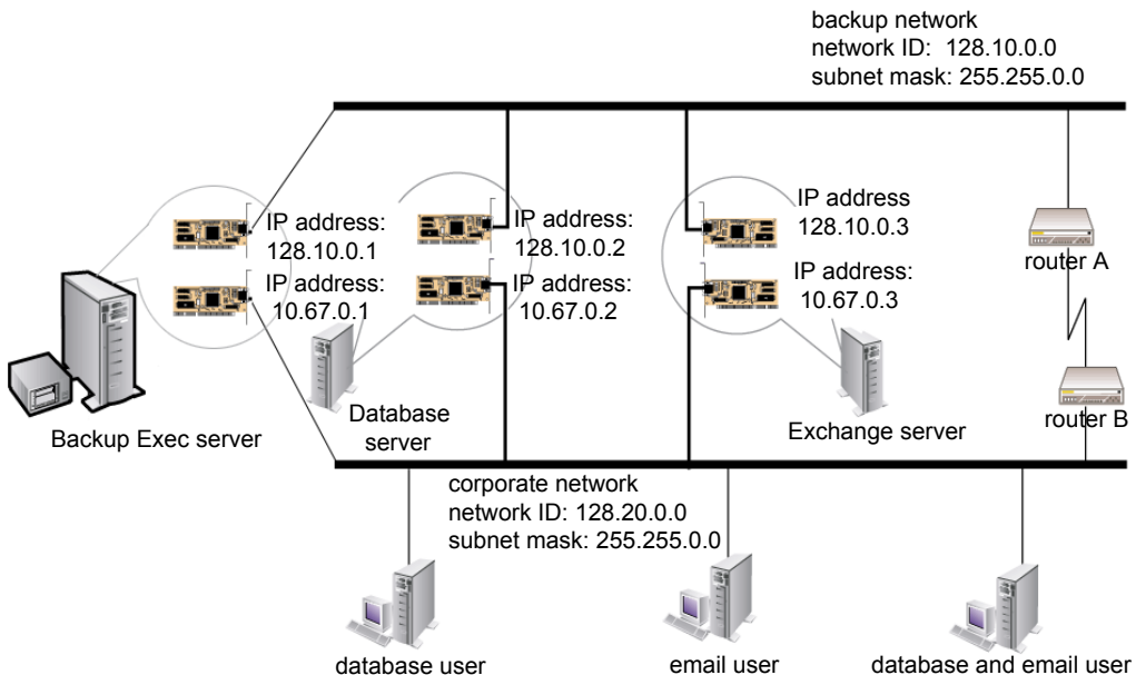
Figure 16-1 Example of backup network
