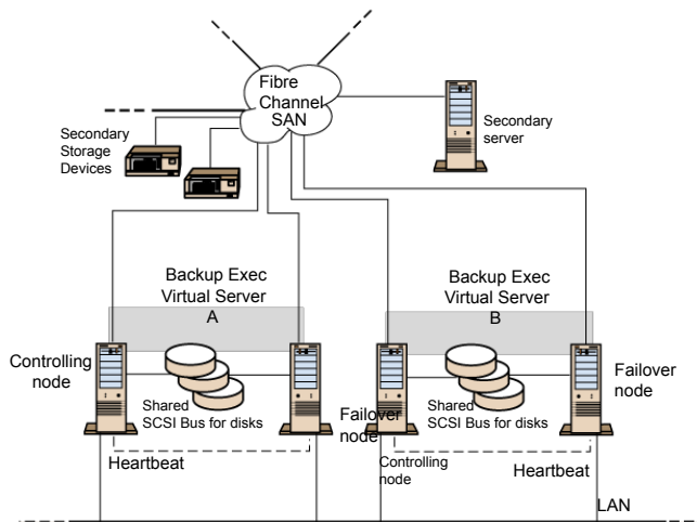
Figure 18-4 Two 2-node Clusters on a Fibre Channel SAN with the Central Admin Server feature
