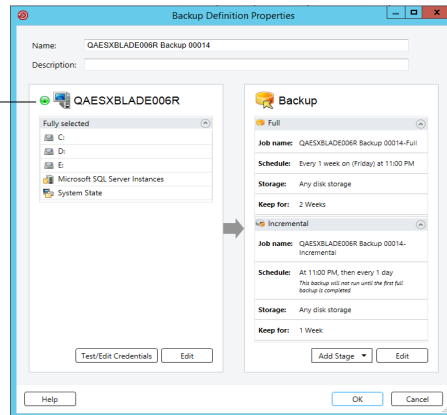
Figure 19-1 Simplified Disaster Recovery indicator is ON in the Backup Definition Properties dialog box
