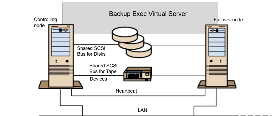
Figure 18-2 Two-node cluster with tape devices on a shared SCSI bus
