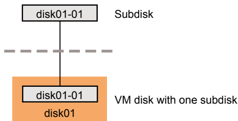
Figure 4-6 Subdisk example
