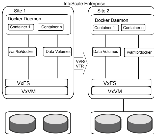
Figure 19-4 Disaster recovery with VVR and VFR technologies
