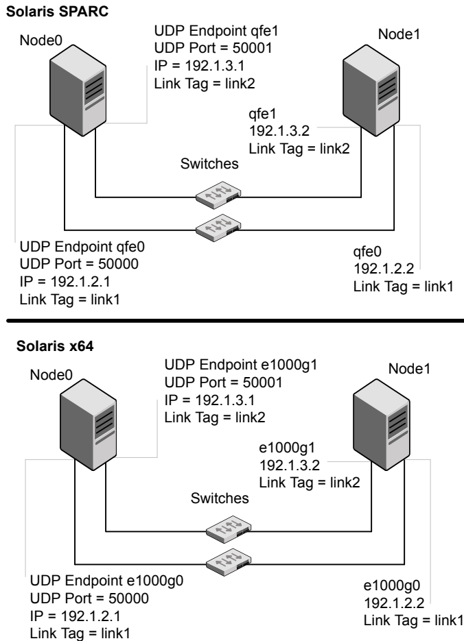
Figure C-1 A typical configuration of direct-attached links that use LLT over UDP
