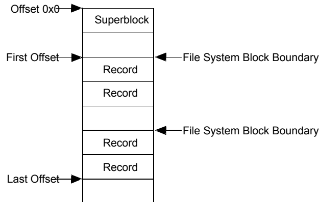
Figure 2-1 FCL file format
