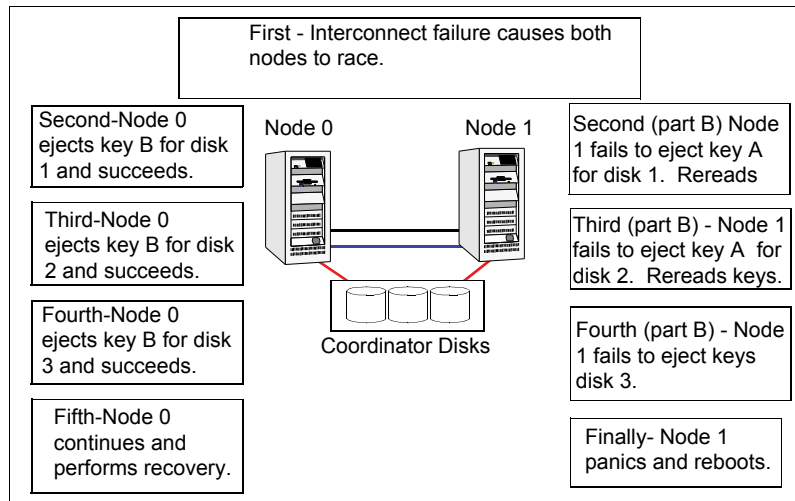
Figure 14-1 Preexisting network partition (split-brain)
