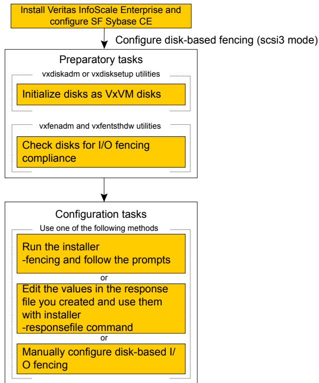
Figure 1-1 Workflow to configure I/O fencing
