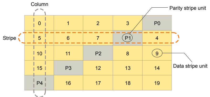
Figure 3-15 Left-symmetric layout
