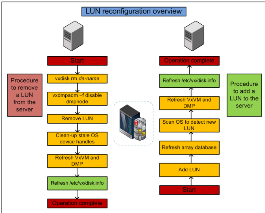
Figure 10-1 LUN reconfiguration overview
