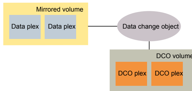
Figure 3-25 Mirrored volume with persistent FastResync enabled
