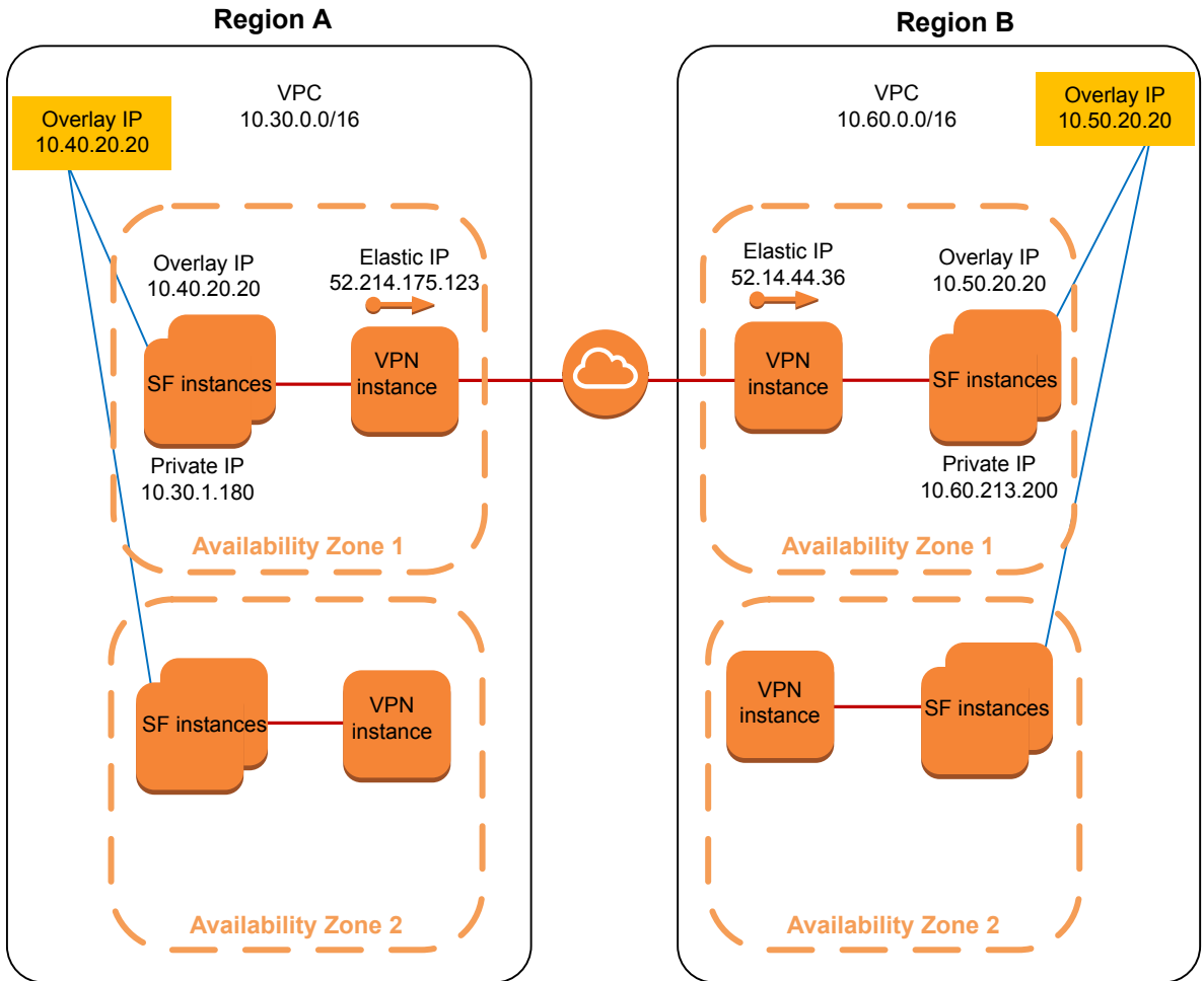
Figure 10-4 Replication across multiple Availability Zones and regions
