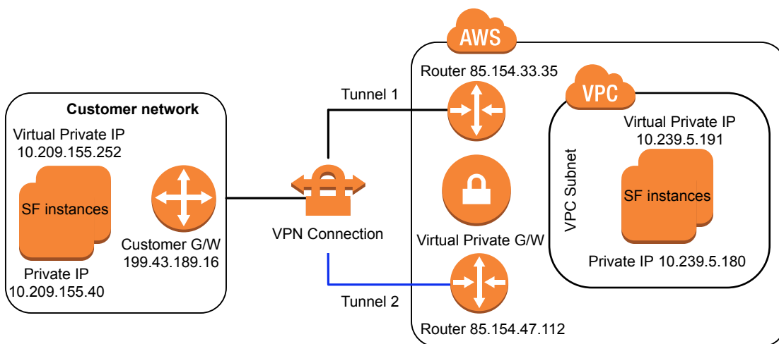
Figure 10-1 Replication from on-premise to cloud
