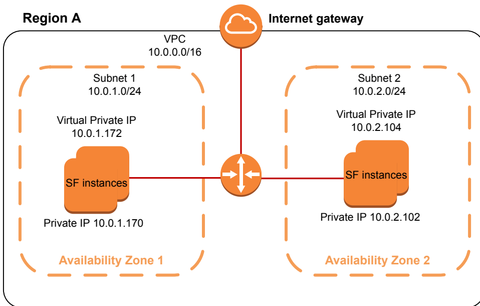
Figure 10-2 Replication across Availability Zones
