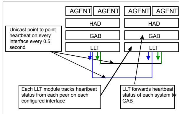
Figure 7-4 Heartbeat in the cluster
