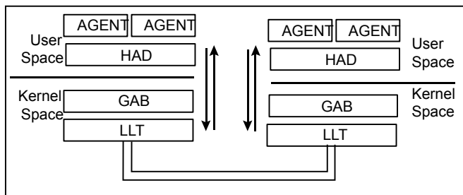
Figure 7-3 Cluster communications with replicated state machine
