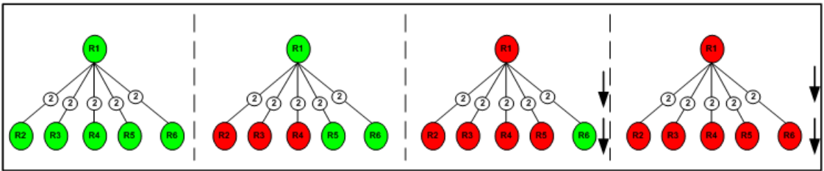
Figure 9-5 Example scenario 4: Resource with atleast resource dependency faults
