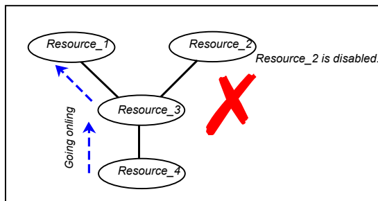
Figure 9-10 Scenario: Child of the disabled resource (Resource_3) is brought online
