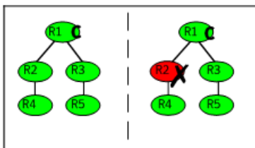
Figure 9-8 Scenario: Resource with a critical parent and FaultPropagation=0
