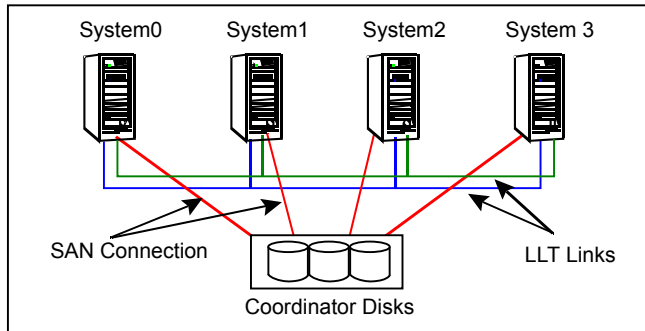
Figure 7-5 Topology of coordinator disks in the cluster
