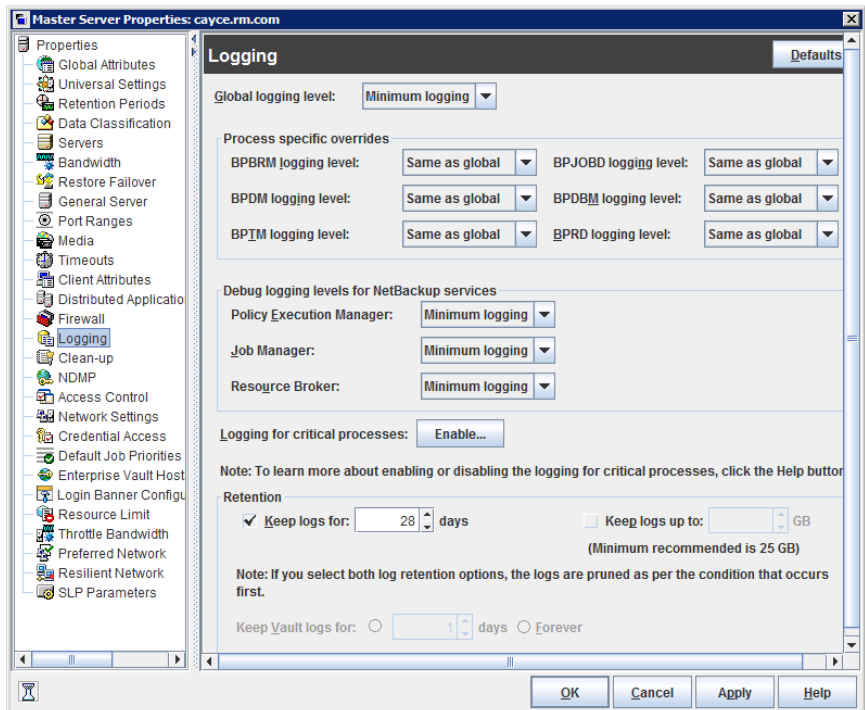
Figure 3-32 Logging dialog box
