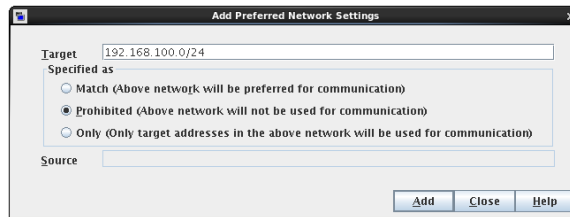
Figure 3-54 Prohibited target example
