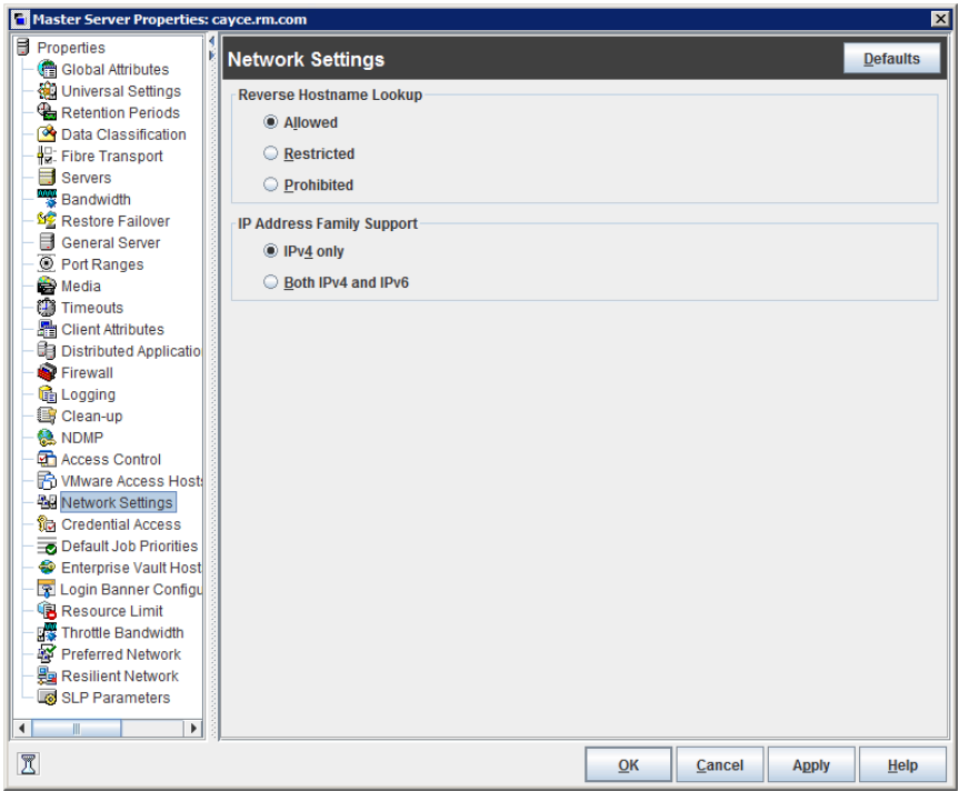
Figure 3-41 Network Settings dialog box
