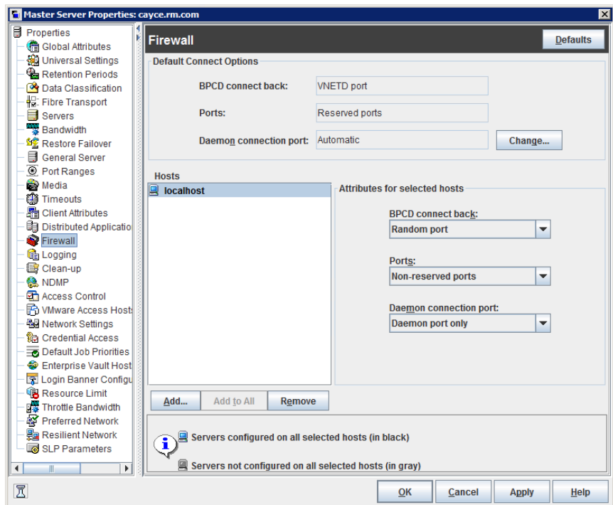
Figure 3-28 Firewall dialog box
