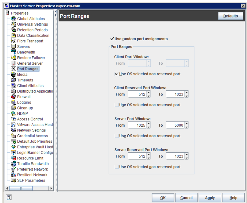
Figure 3-42 Port Ranges dialog box
