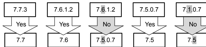
Figure 1-3 Examples of supported and unsupported back-level console configurations
