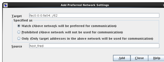
Figure 3-49 Indicating a range of IPv6 networks
