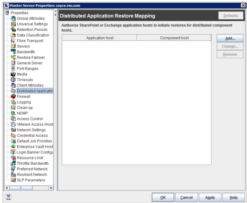
Figure 3-20 Distributed Application Restore Mapping dialog box
