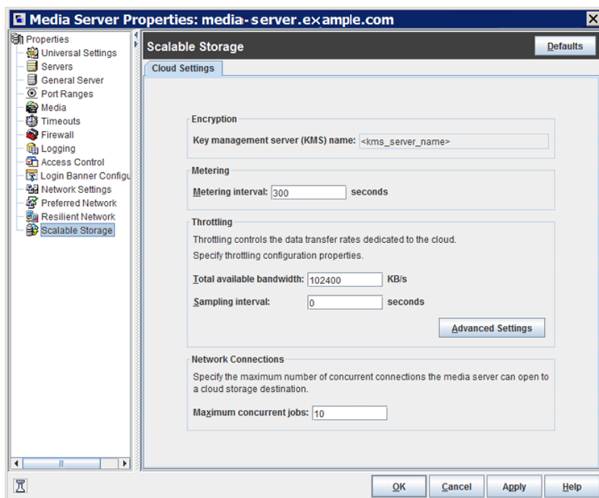
Figure 3-63 Scalable Storage Cloud Settings host properties
