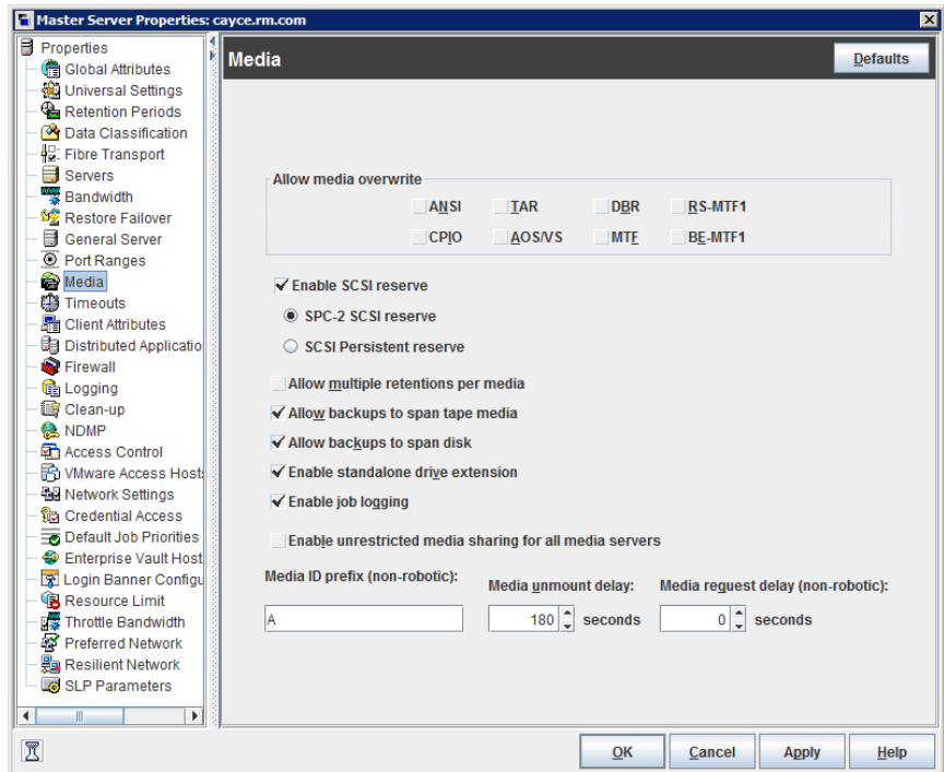
Figure 3-37 Media dialog box
