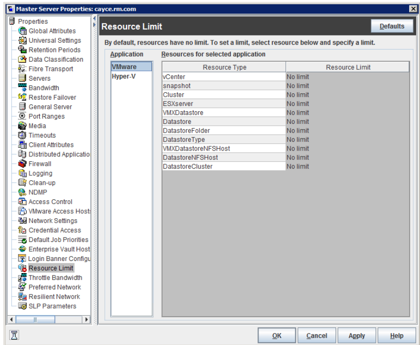
Figure 3-59 Resource Limit dialog box with VMware application selected
