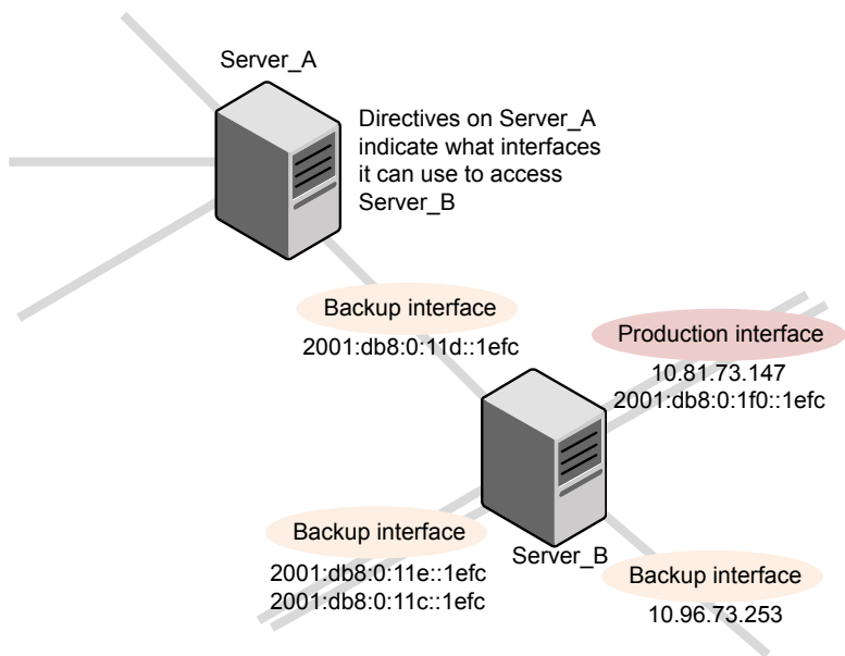
Figure 3-44 Multihomed servers example
