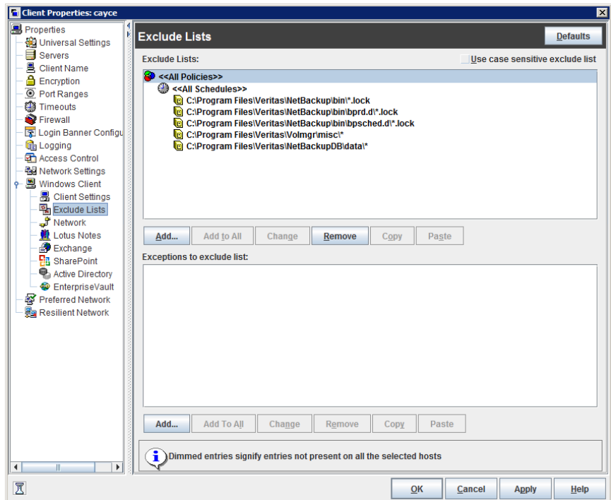
Figure 3-25 Exclude Lists dialog box
