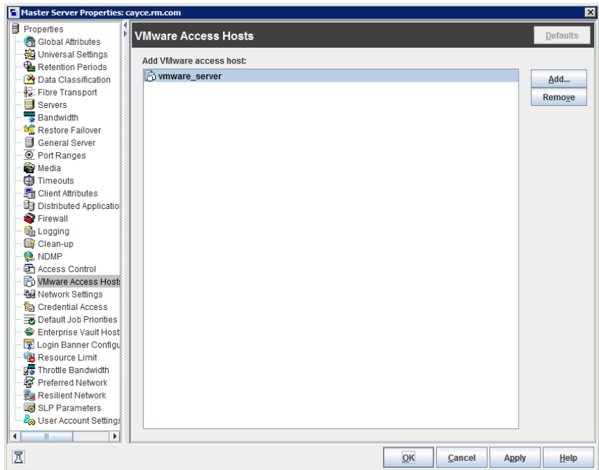
Figure 3-73 VMware Access Hosts dialog box
