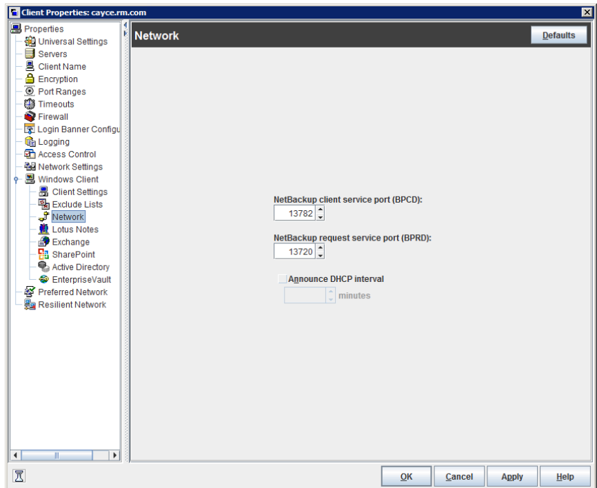
Figure 3-40 Network dialog box
