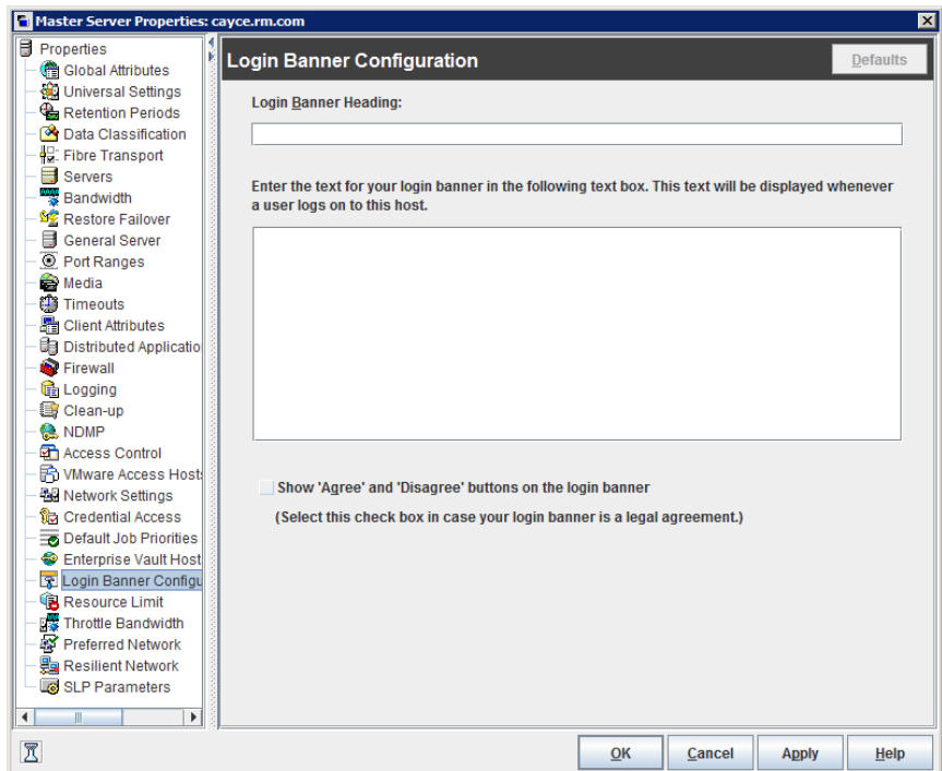
Figure 3-33 Login Banner Configuration dialog box
