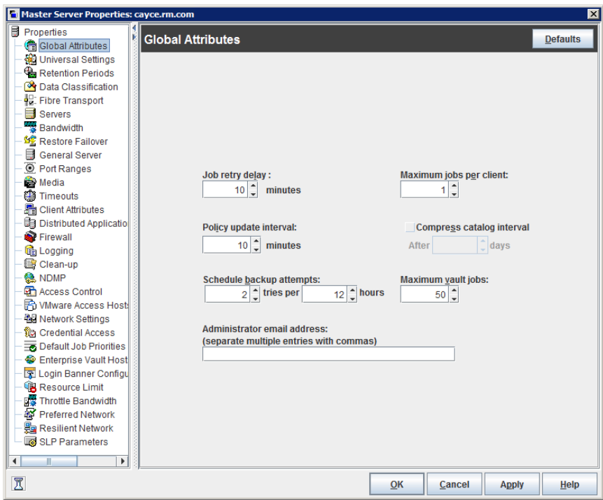
Figure 3-30 Global Attributes dialog box
