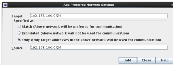
Figure 3-56 Only network selection with the same source binding address
