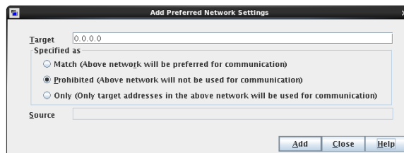
Figure 3-47 Prohibit IPv4 addresses as targets
