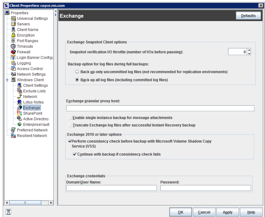
Figure 3-24 Exchange dialog box
