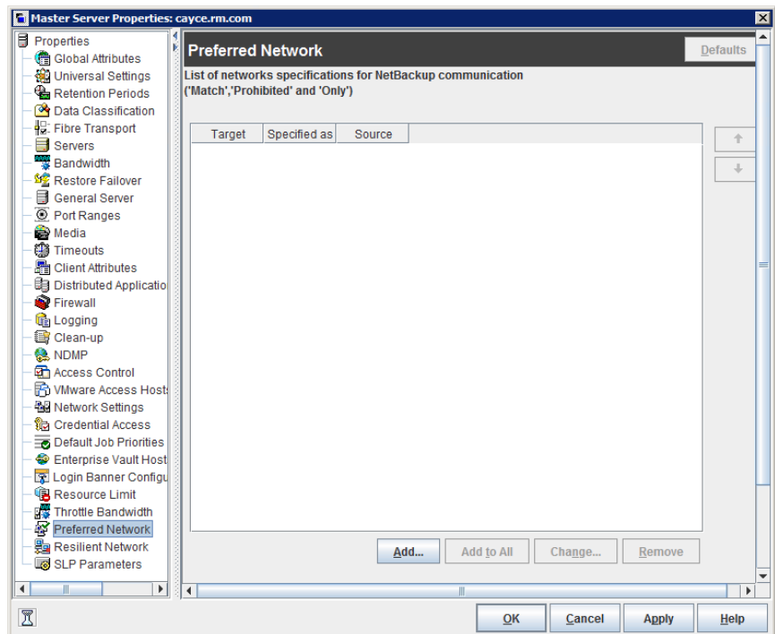
Figure 3-43 Preferred Network dialog box
