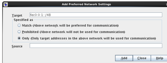
Figure 3-57 Limiting the addresses, without any source binding
