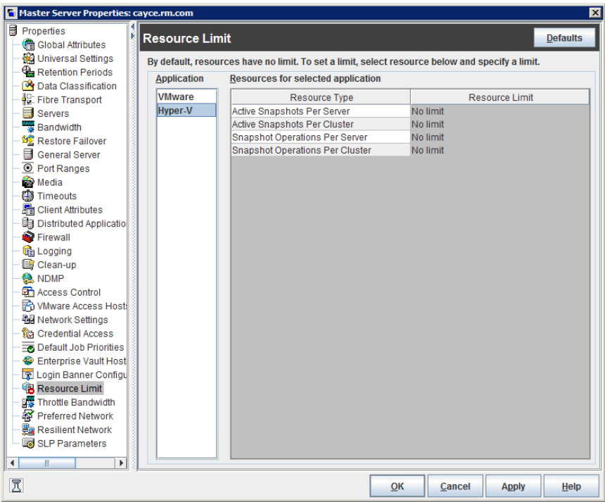
Figure 3-60 Resource Limit dialog box with Hyper-V application selected
