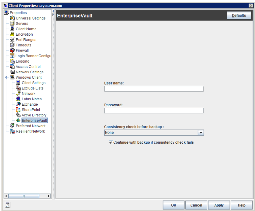
Figure 3-22 Enterprise Vault dialog box
