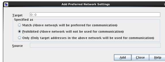
Figure 3-50 Prohibit IPv6 addresses as targets
