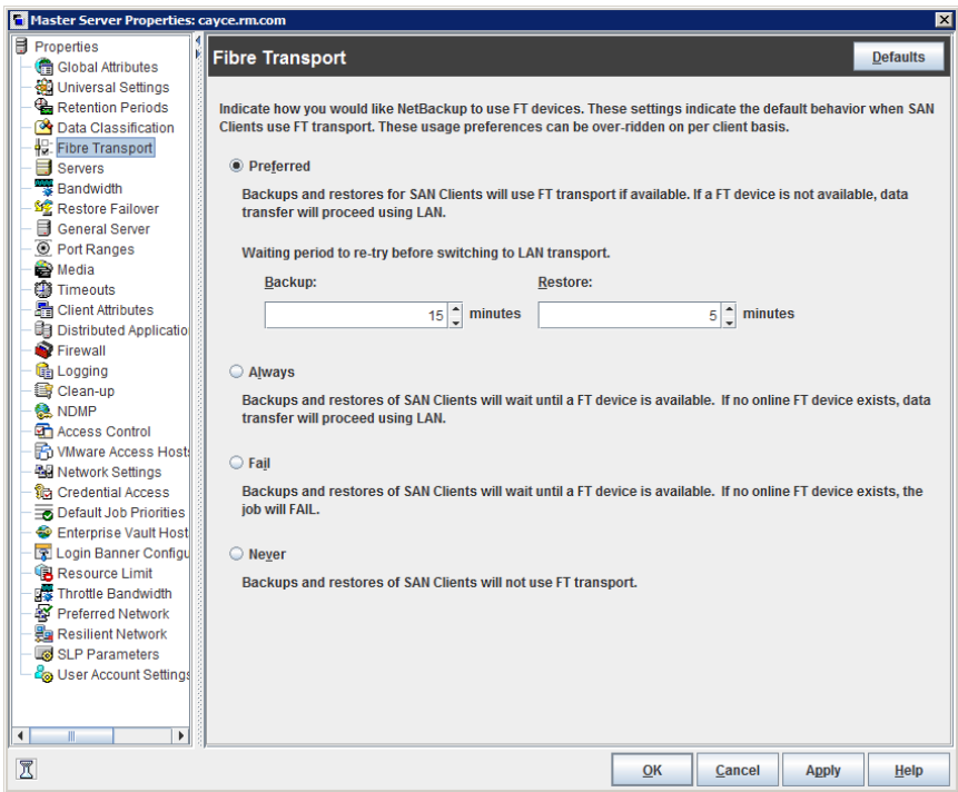
Figure 3-27 Fibre Transport host properties for a master server
