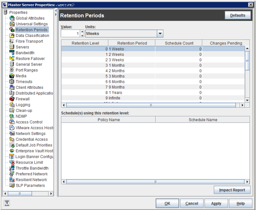
Figure 3-62 Retention Periods dialog box
