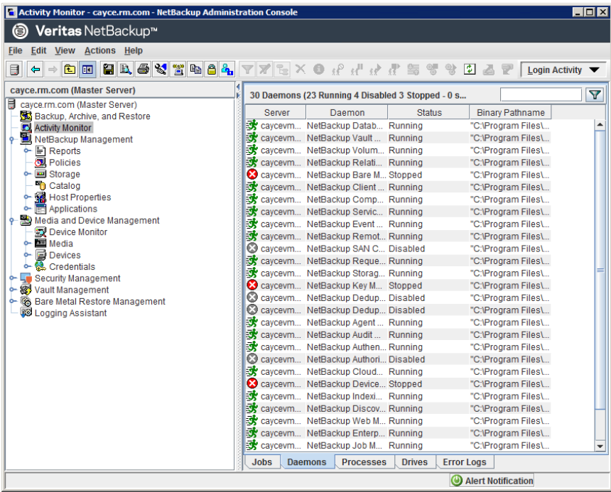
Figure 26-2 The Daemons tab in the Activity Monitor
