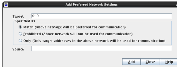
Figure 3-48 Match IPv6 addresses as targets
