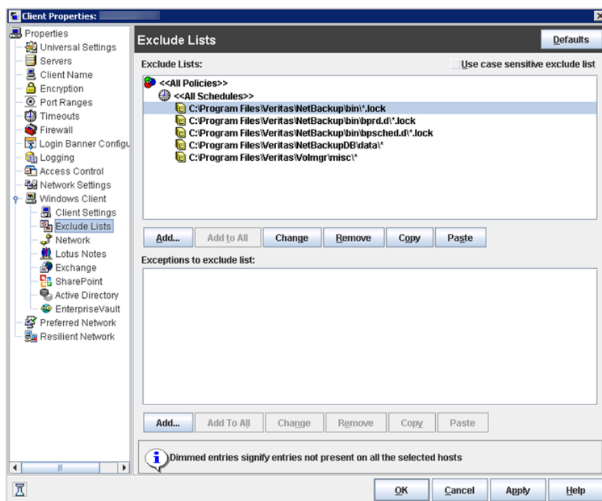
Figure 7-1 Exclude list for two Exchange databases
