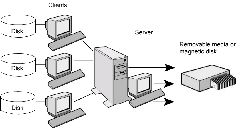
Figure 20-13 Multiplexed backups
