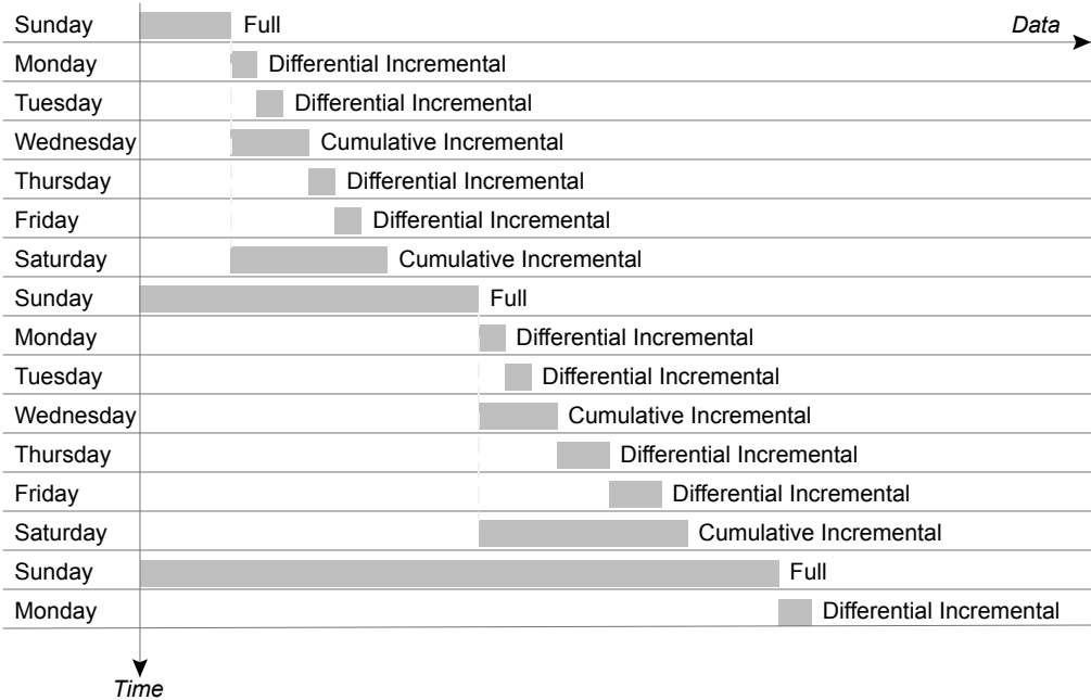
Figure 20-17 Schedule coverage
