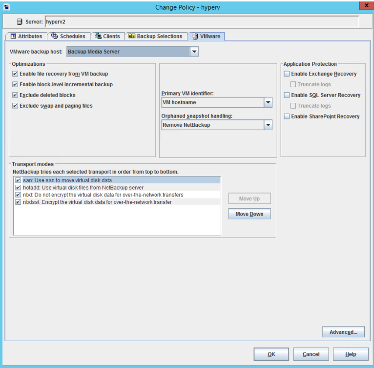
Figure 20-31 VMware tab
