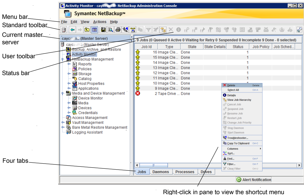
Figure 26-1 Activity Monitor
