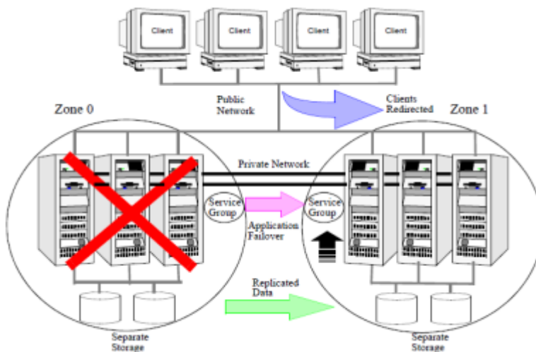
Figure 1-2 Failover in a replicated data cluster
