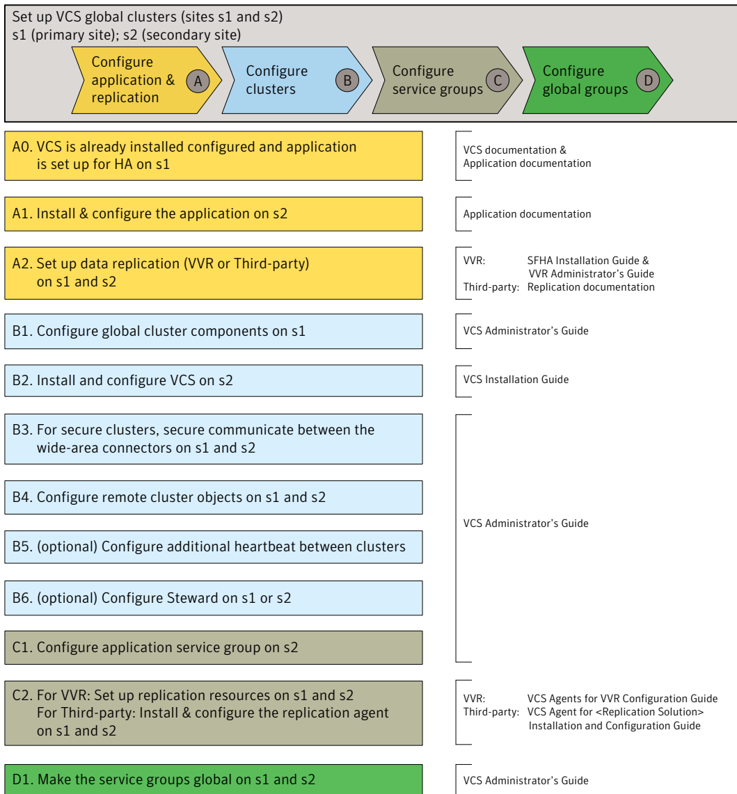
Figure 15-4 High-level workflow to set up VCS global clusters
