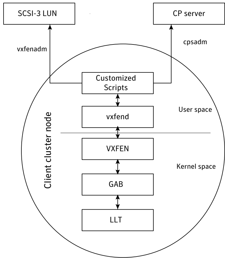
Figure 9-6 Customized fencing
