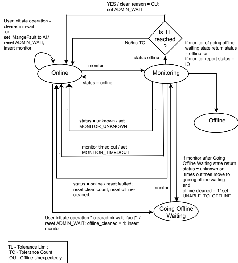
Figure 10-14 Resource fault (unexpected offline): ManageFaults attribute = NONE
