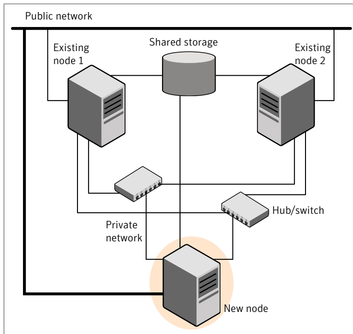
Figure 35-1 Adding a node to a two-node cluster using two switches
