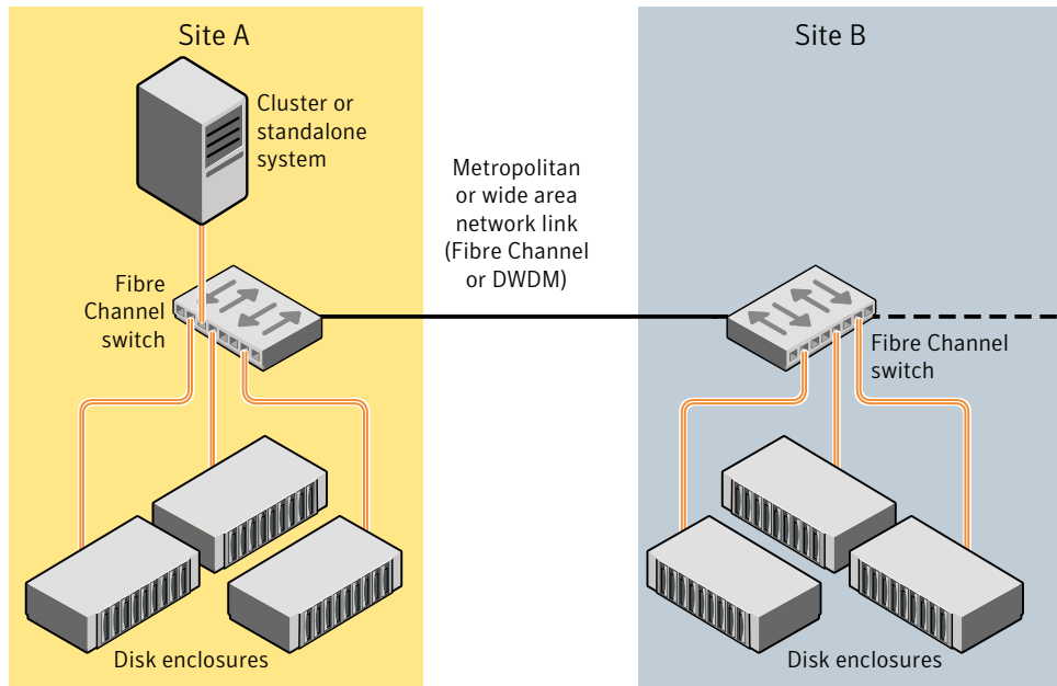
Figure 20-3 Example of a two-site configuration with remote storage only
