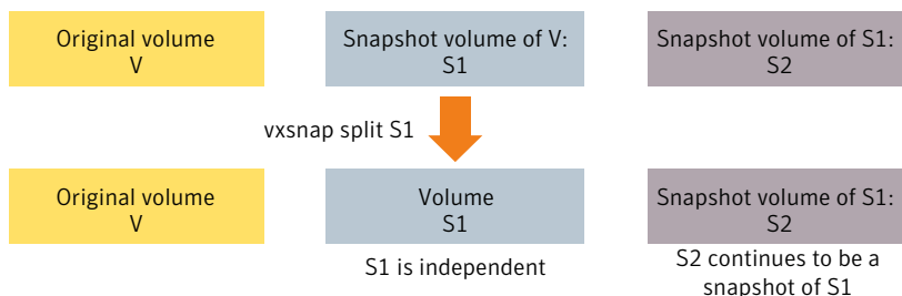
Figure 27-7 Splitting snapshots
