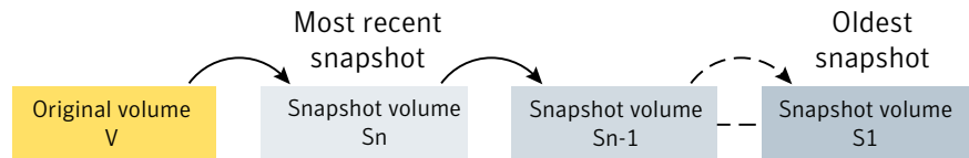
Figure 27-3 Snapshot cascade
