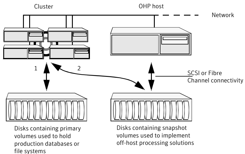
Figure 26-6 Example implementation of an off-host point-in-time copy solution using a separate OHP host
