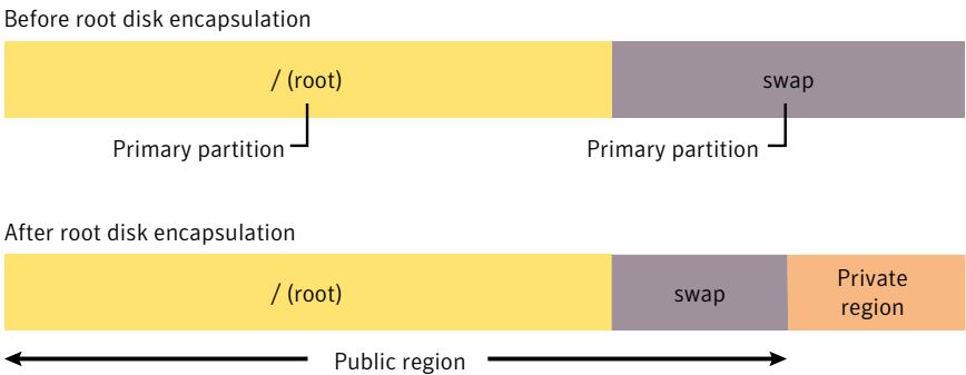
Figure 42-2 Root and swap configured on two primary partitions, and no free space
