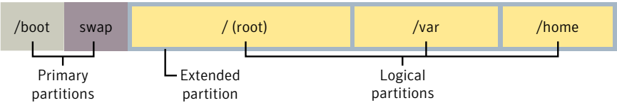
Figure 42-10 Boot and swap configured on two primary partitions, and no free space
