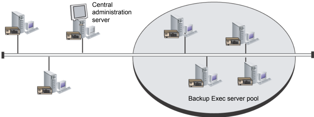
Figure K-3 An example of a CASO-configured Backup Exec server pool inside a corporate network
