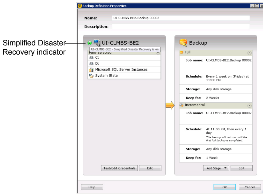
Figure 4-3 Simplified Disaster Recovery indicator is ON in the Backup Definition Properties dialog box
