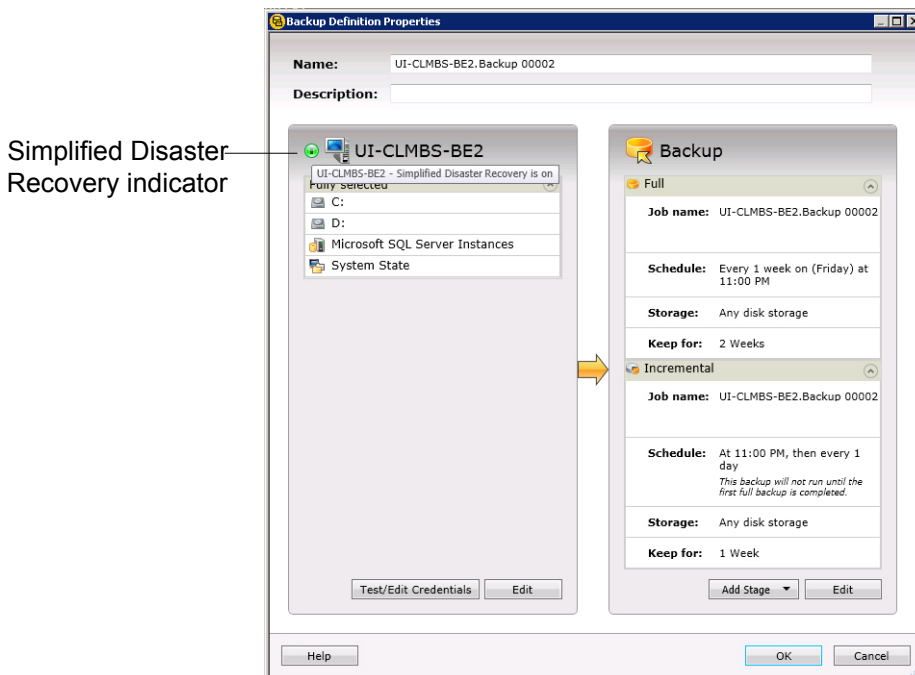
Figure 4-4 Simplified Disaster Recovery indicator is ON in the Backup Definition Properties dialog box
