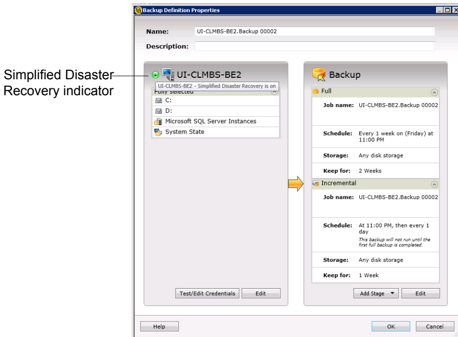
Figure 18-1 Simplified Disaster Recovery indicator is ON in the Backup Definition Properties dialog box
