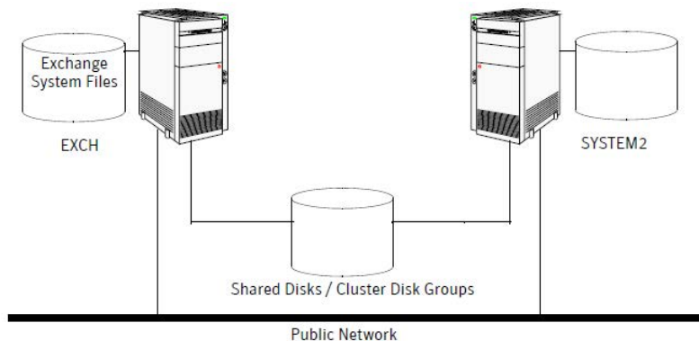
Figure 2-4 Standalone initial configuration
