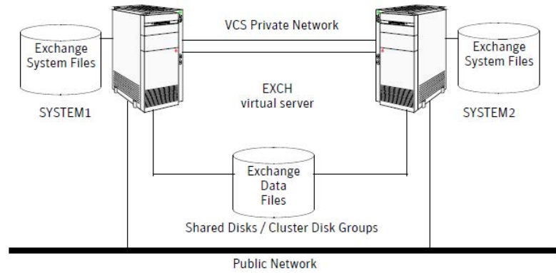
Figure 2-5 Standalone to active-passive completed configuration
