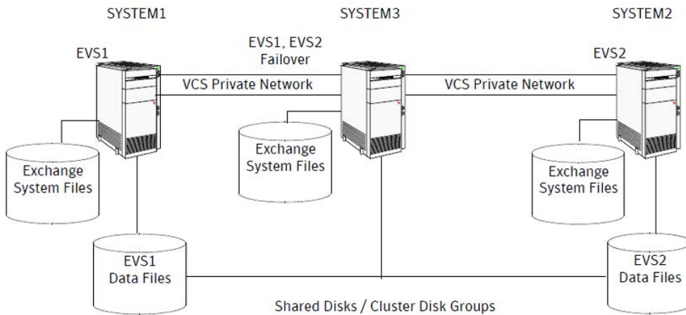
Figure 2-2 Three-node cluster in an any-to-any configuration
