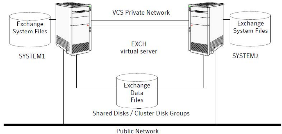
Figure 2-7 Standalone to active-passive completed configuration
