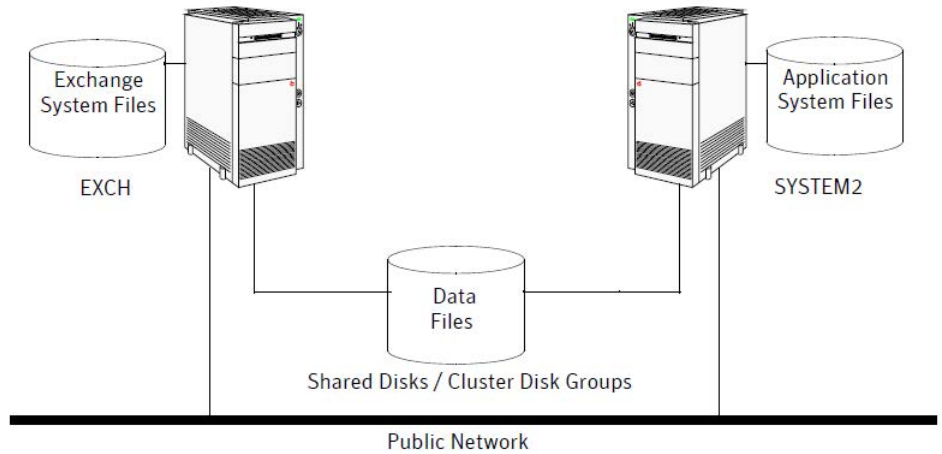
Figure 2-6 Standalone initial configuration with a cluster
