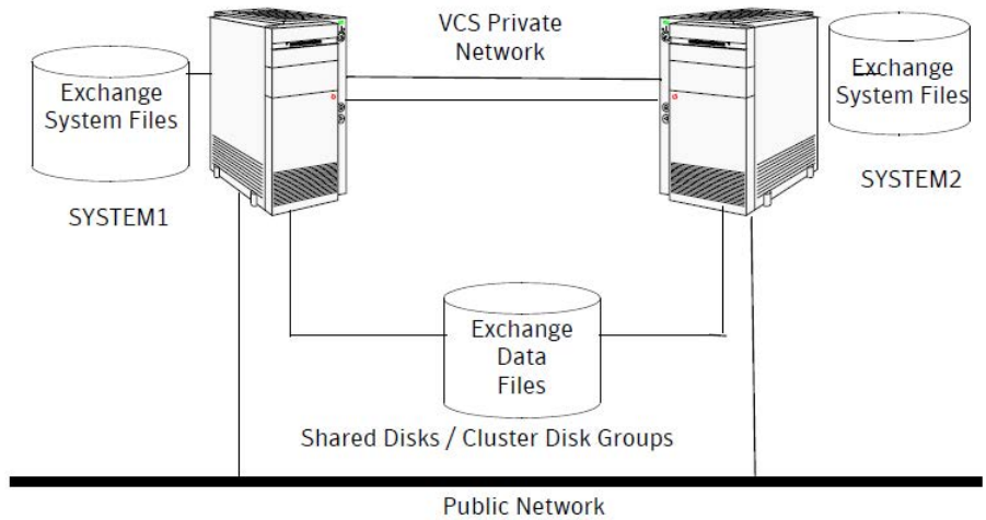
Figure 2-1 Active-passive failover configuration
