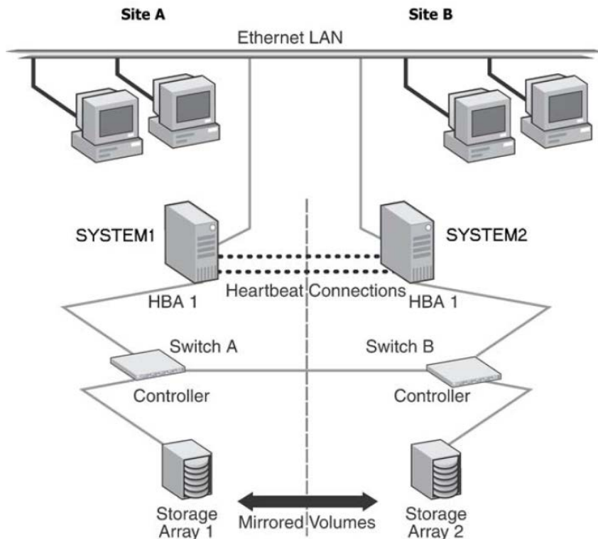
Figure 2-3 Campus cluster: Active-Passive configuration
