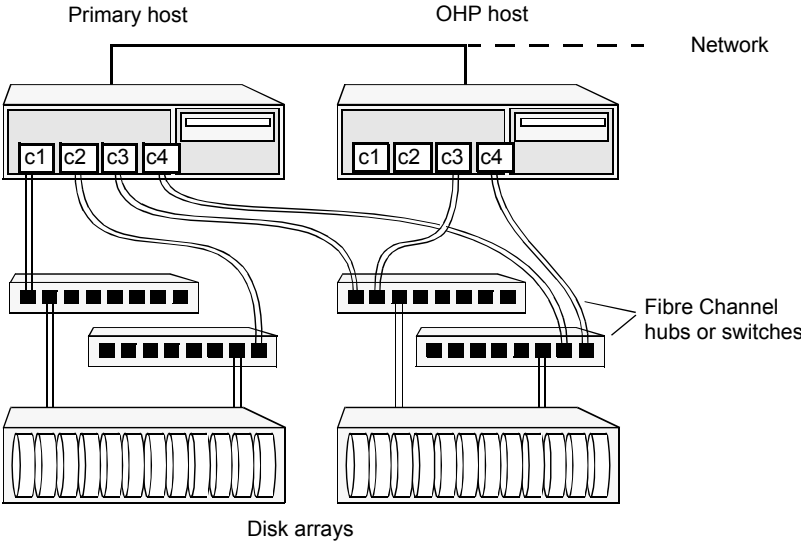
Figure 23-4 Example connectivity for off-host solution using redundant-loop access
