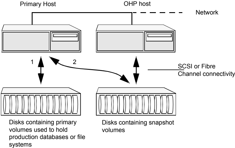
Figure 23-3 Example implementation of an off-host point-in-time copy solution
