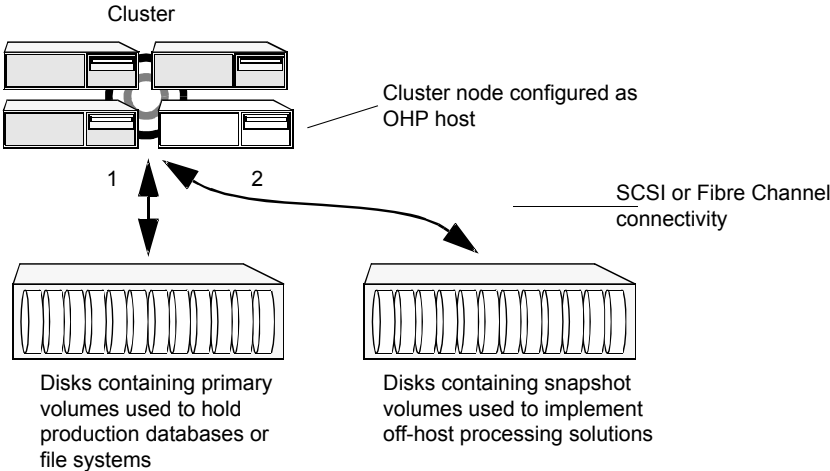
Figure 23-5 Example implementation of an off-host point-in-time copy solution using a cluster node
