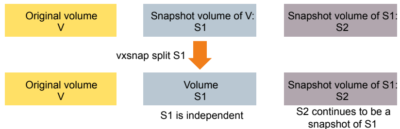
Figure 24-7 Splitting snapshots
