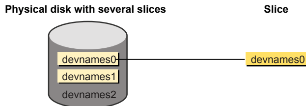
Figure 3-2 Slice example
