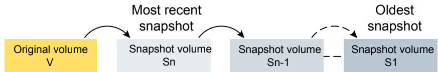
Figure 24-3 Snapshot cascade
