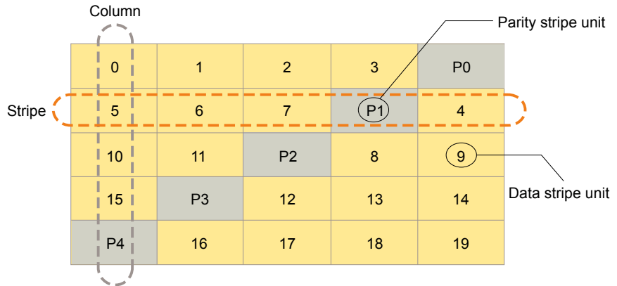
Figure 3-16 Left-symmetric layout
