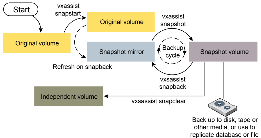
Figure 24-1 Third-mirror snapshot creation and usage
