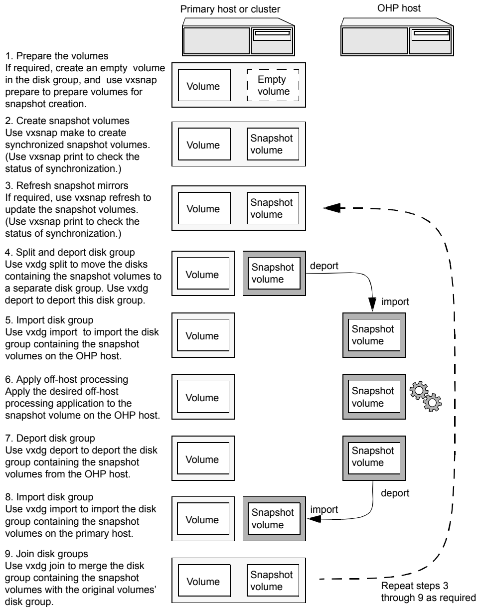
Figure 23-7 Implementing off-host processing solutions
