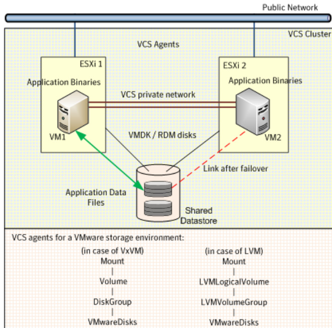
Figure 16-1 Typical generic applications cluster configuration in a VMware virtual environment
