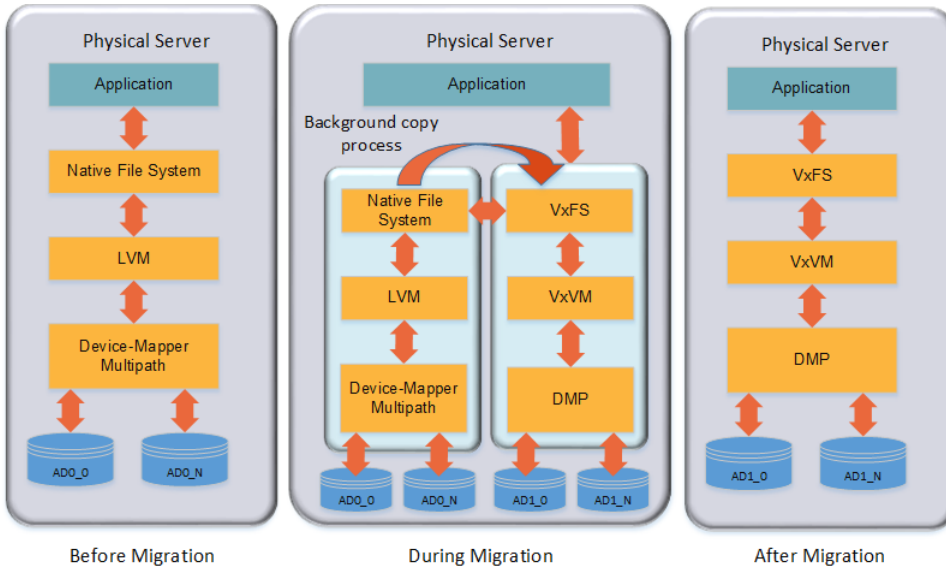
Figure 16-1 Migration process
