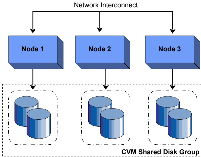
Figure 13-1 Flexible Storage Sharing Environment
