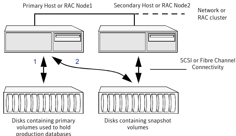
Figure 10-2 Example of an off-host or Oracle RAC Database FlashSnap solution
