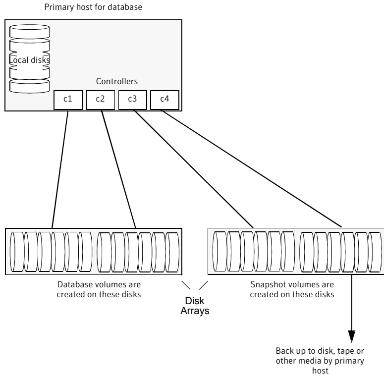
Figure 10-5 Example system configuration for database backup on the primary host
