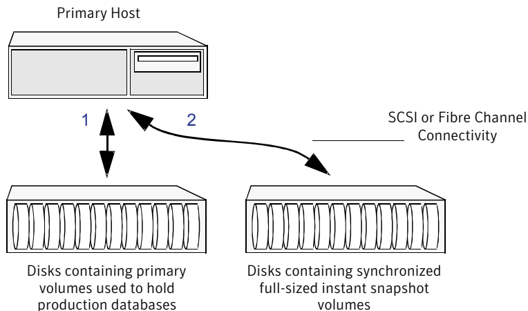
Figure 10-1 Example of a Database FlashSnap solution on a primary host
