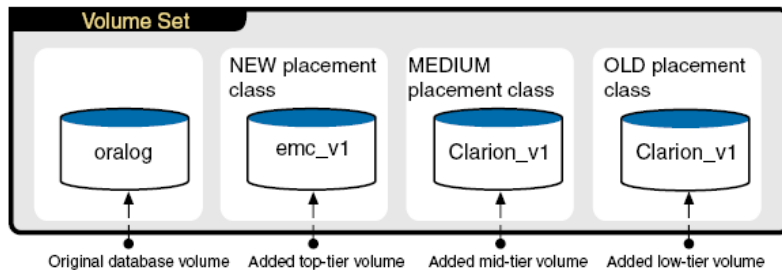
Figure 9-1 Database storage configuration suitable for automatic relocation of archive and Flashback logs
