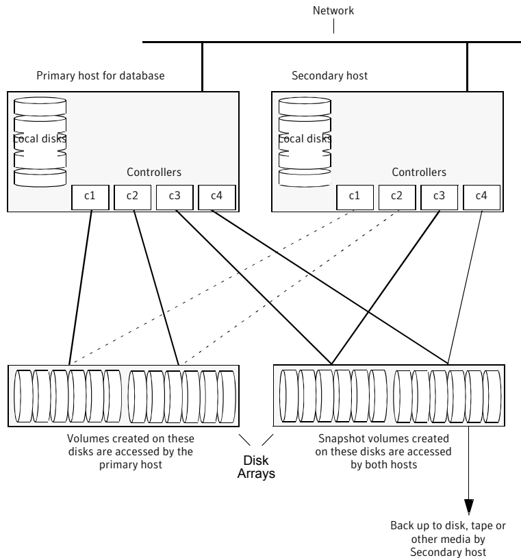
Figure 10-6 Example system configuration for database backup on a secondary host
