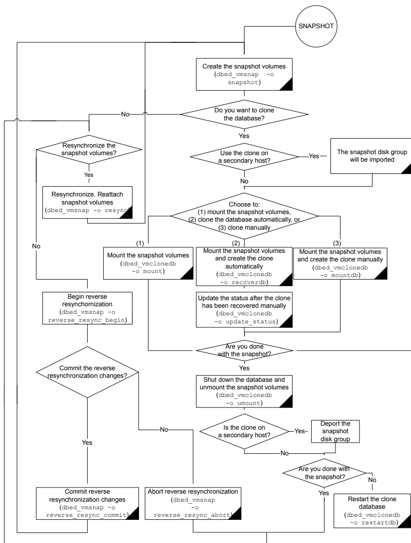
Figure 10-4 Database FlashSnap process
