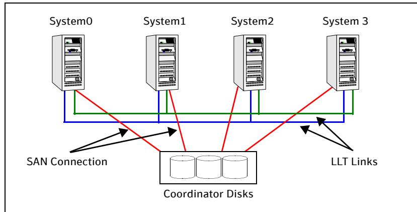
Figure 11-3 Topology of coordinator disks in the cluster
