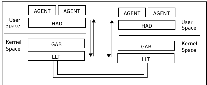
Figure 11-1 Cluster communications with replicated state machine
