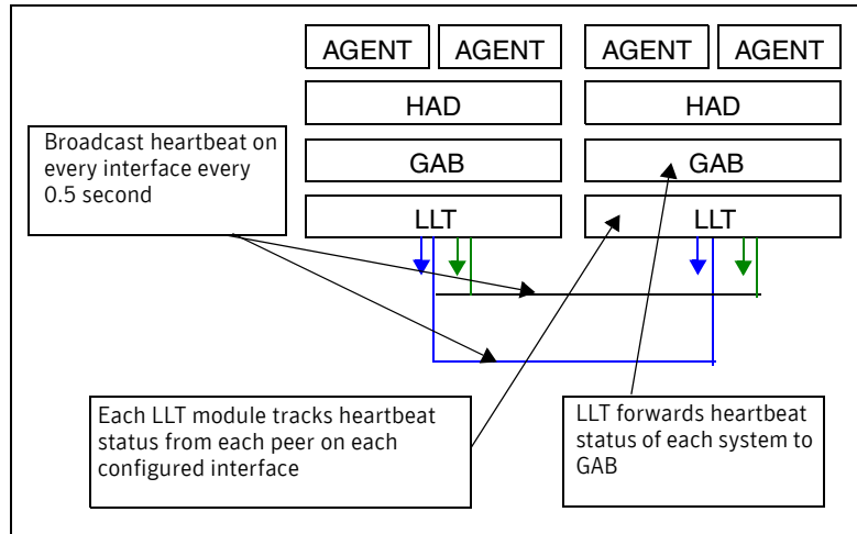
Figure 11-2 Heartbeat in the cluster
