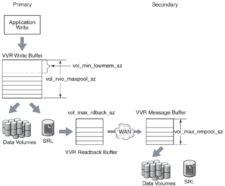
Figure 18-2 How VVR uses buffers during a readback
