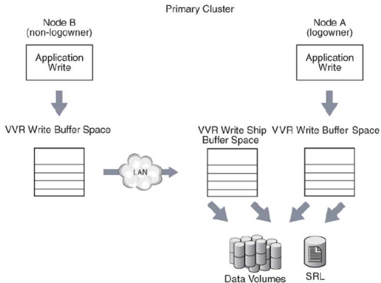
Figure 18-3 How VVR uses buffers on a Primary in a shared disk group for synchronous RLINKs
