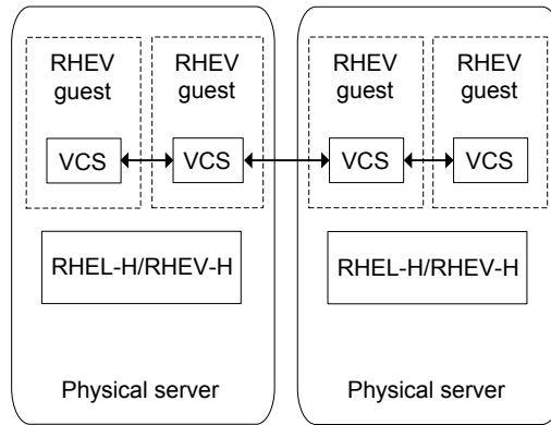
Figure 4-8 Cluster Server in the RHEV guest
