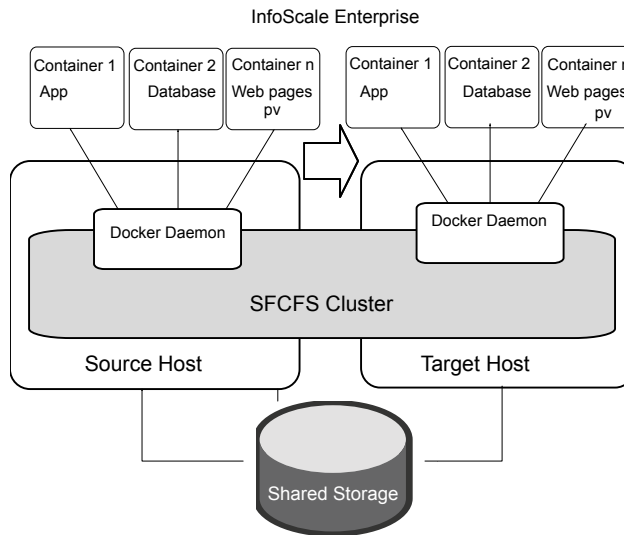
Figure 20-3 Migration of Docker Daemon and Docker Containers
