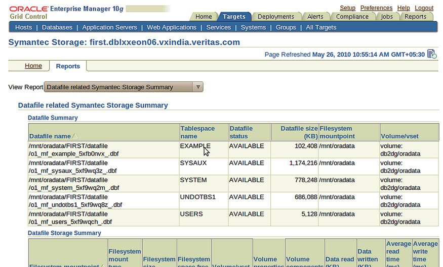
Figure A-8 Datafile report
