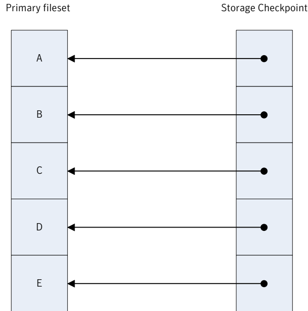
Figure 15-3 Initializing a Storage Checkpoint
