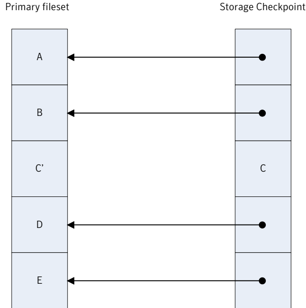
Figure 15-4 Updates to the primary fileset
