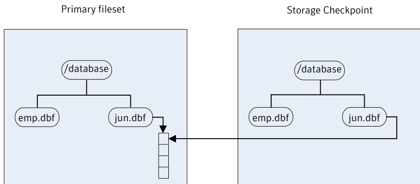
Figure 15-2 Primary fileset and its Storage Checkpoint
