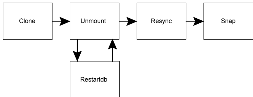
Figure 17-4 Resynchronizing Mirror Volumes
