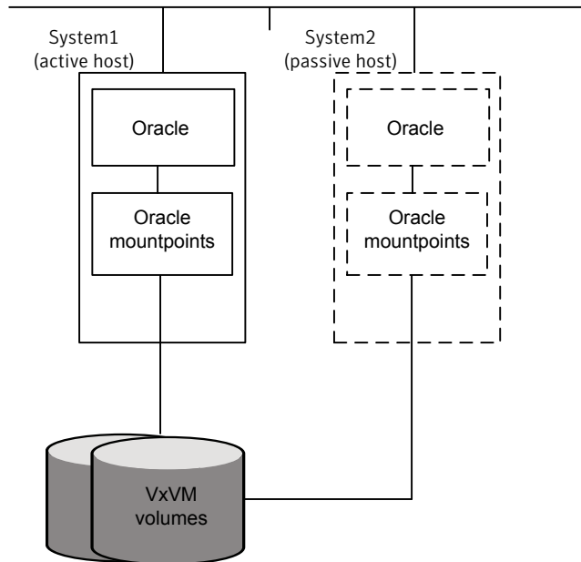
Figure 2-3 Oracle single instance with SFHA
