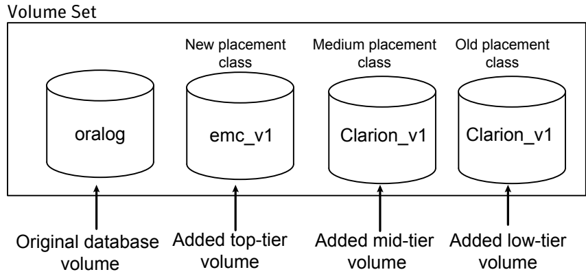
Figure 24-1 Database storage configuration suitable for automatic relocation of archive and Flashback logs
