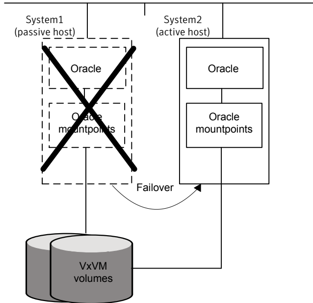
Figure 2-4 Oracle single instance with SFHA failover setup
