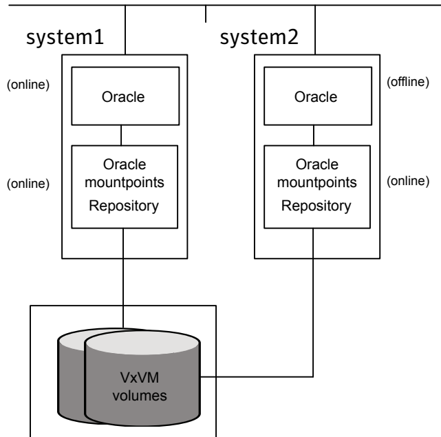
Figure 2-5 SF Cluster File System HA setup example
