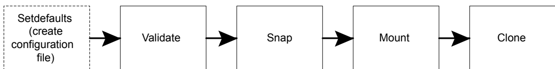
Figure 17-3 Creating a Clone - Workflow
