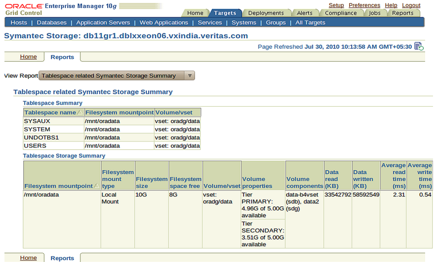
Figure A-7 Tablespace report
