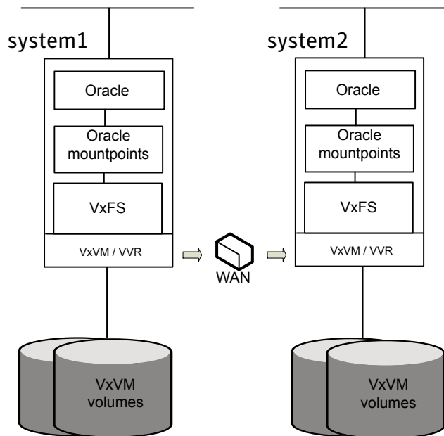
Figure 2-8 Oracle single instance - Storage Foundation with VVR
