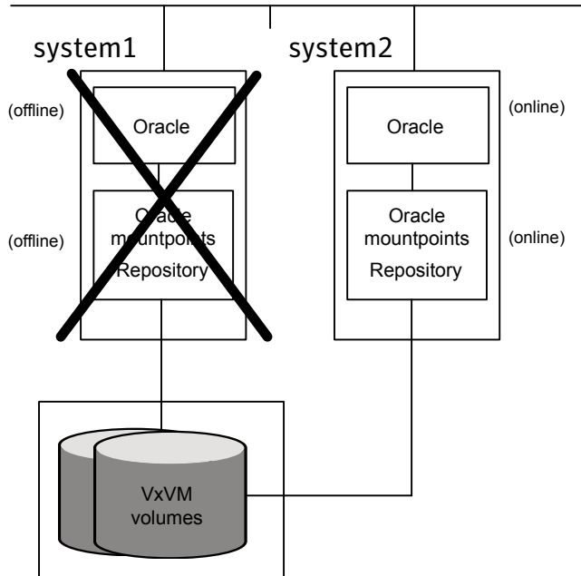
Figure 2-6 SFCFS HA failover example
