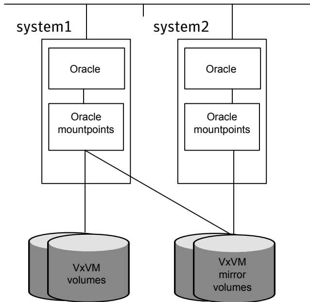
Figure 2-2 Oracle single instance off-host setup with Storage Foundation environment
