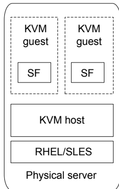
Figure 5-2 Storage Foundation in the guest
