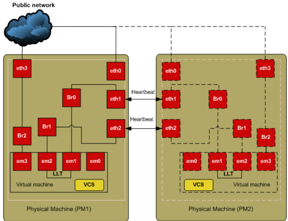
Figure 6-3 Network configuration for VM- VM cluster
