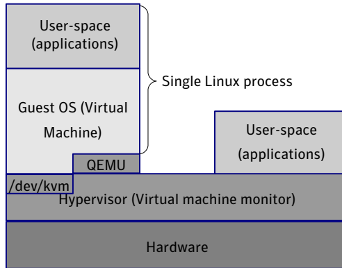
Figure 2-1 KVM process
